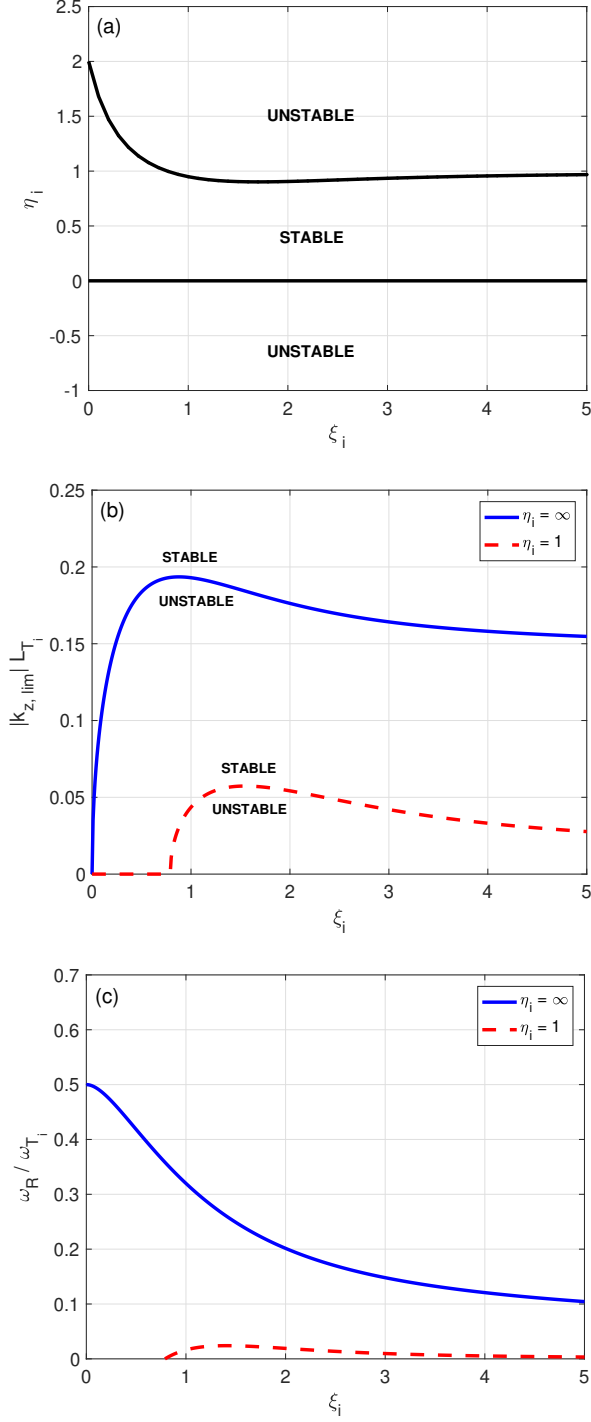
Figure 1.13: Conditions of marginal stability for the slab-ITG instability: a) Critical \eta_i value, b) upper limit on |k_z| , and c) real frequency \omega_R as a function of \xi_i = (k_y \lambda_{Li})^2 , for \eta_i = \infty and \eta_i = 1 . For this figure one assumed T_e = T_i .
