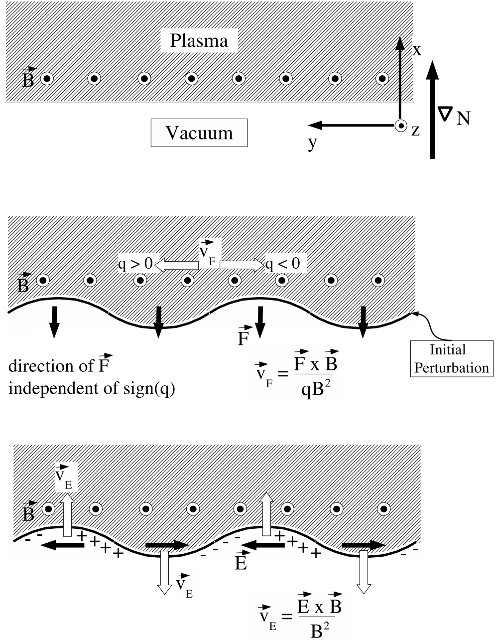
Figure 1.7: Basic mechanism of the interchange instability: One considers a magnetised plasma with density gradient \nabla N , and submitted to a charge independent force \vec{F} perpendicular to \vec{B} . In the presence of an initial density perturbation perpendicular to \vec{B} , the drifts \vec{v}_F = (\vec{F} \times \vec{B}) / (qB^2) lead to a charge separation. The corresponding electric field \vec{E} induces charge independent drifts \vec{v}_E = (\vec{E} \times \vec{B}) / B^2 , which amplify the perturbation, thus leading to an instability.
