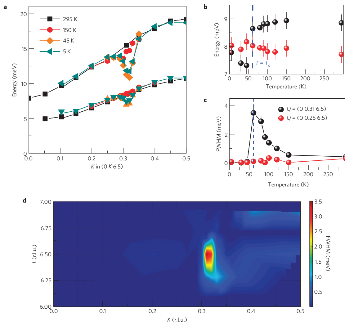
Figure 4 | Temperature dependence of the phonon dispersion. a , Dispersion of the two low-energy phonons in the Z-T direction at T = 295, 150, 45 and 5 K. b,c , Temperature dependence of the acoustical phonon energy and FWHM, respectively, at Q = (0\ 0.25\ 6.5) (red dots) and Q = (0\ 0.31\ 6.5) (black dots). In both panels, error bars represent the fit uncertainty. d , Momentum dependence of the intrinsic FWHM of the transverse acoustic phonon at T = T_c .
