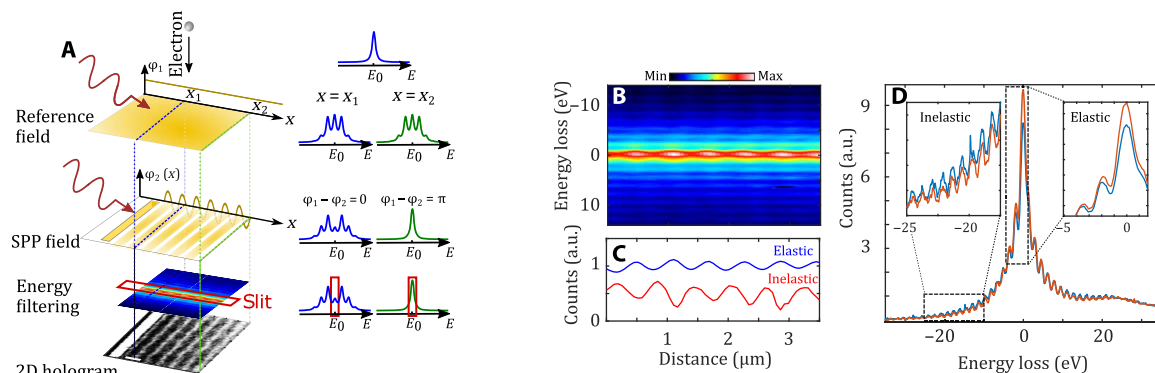
Fig. 3. Principle of spatially separated electron holography. (A) The initial energy distribution of the electron beam is a function of energy that is singly peaked at E = E_0 (right). Interaction with the reference field produces coherent superposition states with energies E = E_0 \pm \hbar\omega . The ensuing interaction with an SPP depends on the relative phase between SPP and reference fields, which results in a position-dependent electron energy distribution. The elastic part of the electron spectrum is then used to form the 2D hologram. The spectra on the right are simulations from an analytical model (see Materials and Methods). (B) Hybrid energy-space map (spectrogram) of the electrons after interaction with the two fields, as schematized in (A). (C) Spatial profiles of the normalized intensity for elastic (blue curve) and inelastic (red curve) electrons, as obtained from (B) by energy-averaging from -1 to 1 eV for the elastic contribution and from -27 to -12 eV for the inelastic one. (D) Energy profiles at the maximum and minimum of the spatial modulation shown in (B), averaged over four periods.
