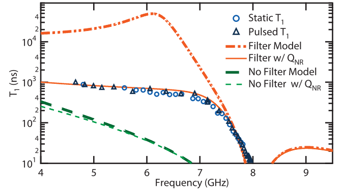
FIG. 2. (Color) Qubit T_1 as a function of frequency measured with two methods and comparison to various models. The first method is a static measurement (circles): the qubit is excited and measured after a wait time \tau . The second (triangles) is a dynamic measurement: the qubit frequency is tuned with a fast flux pulse to an interrogation frequency, excited, and allowed to decay for \tau , and then returned to its operating frequency of 5.16 GHz and measured. This method allows for accurate measurement even when T_1 is extremely short. Measurements using the two methods show near perfect overlap. The top dashed curve is the predicted T_1^{Purcell} , while solid curve includes also nonradiative internal loss with best-fit Q_{NR} = 2\pi f T_1^{NR} \approx 27\,000 . The two lower curves correspond to an unfiltered device with the same C_{in} , C_{out} , and \omega_c , with and without the internal loss. In this case, the Purcell filter gives a T_1 improvement by up to a factor of \sim 50 (6.7 GHz).
