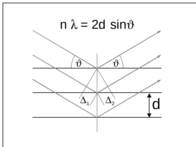
Fig. 2: Schematic representation of the Bragg condition.
