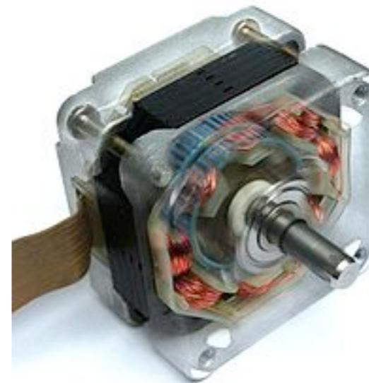
Digital version with static coils and magnet that turns
