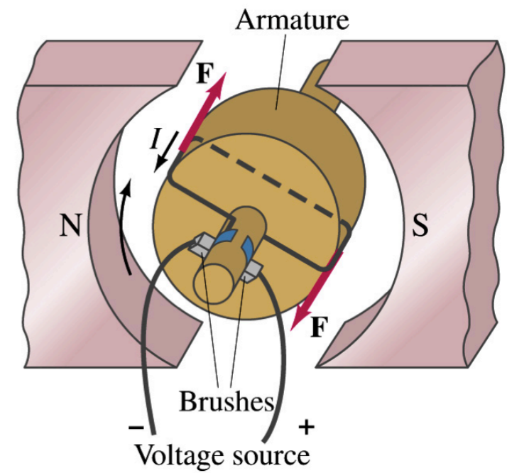
Electromotor
