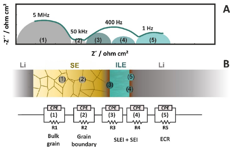
Figure 28. (A) Nyquist plot of \text{Li}|\text{ILE}|\text{SE}|\text{Li} (green line) cell with its respective fit and characteristic peak frequencies. (B) Schematic of the \text{Li}|\text{ILE}|\text{SE}|\text{Li} cell and the equivalent circuit used for fitting the impedance data. Li, Lithium electrode, SE, solid electrolyte, ILE, ionic liquid electrolyte, ECR, electrochemical reaction. Adapted with permission from ref 85. Copyright 2021 Wiley.
