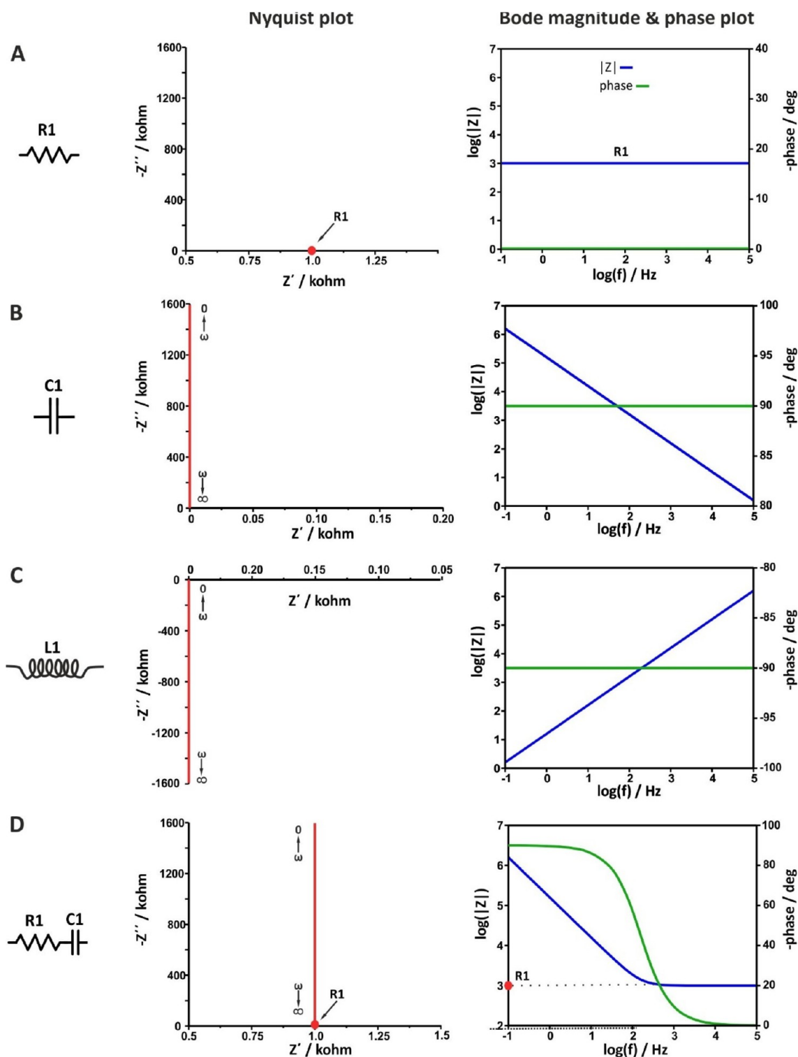
Figure 8. Nyquist, Bode magnitude and phase angle plots of some model circuits. R1 = 1 kΩ.
