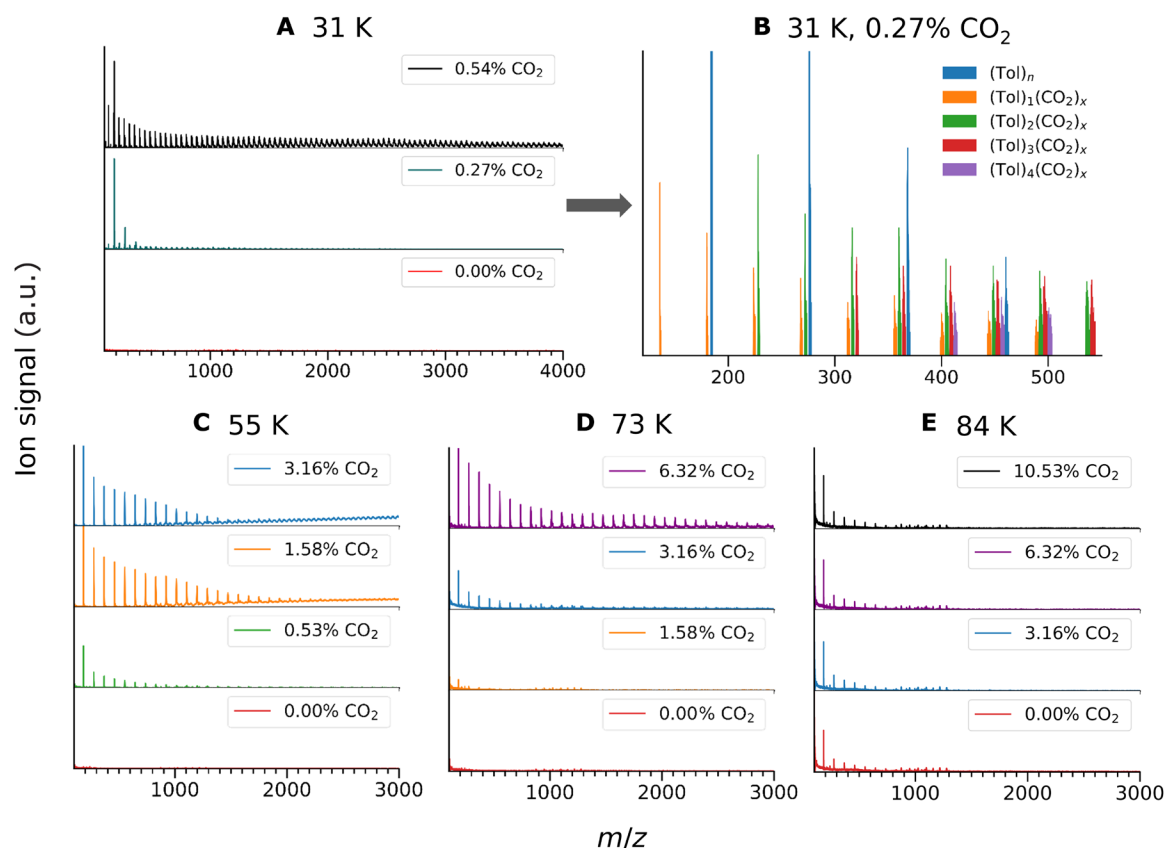
Fig. 4. Temperature dependence of binary toluene- \text{CO}_2 nucleation. The mass spectra are recorded at flow temperatures T_F of (A and B) 31 K, (C) 55 K, (D) 73 K, and (E) 84 K at a constant L_{NS} = 100 mm and for constant toluene concentrations. (B) A zoomed-in segment of the mass spectrum in (A) for 0.27% \text{CO}_2 . The color code indicates the composition of the (\text{Tol})_j(\text{CO}_2)_x clusters. Detailed experimental conditions are specified in table S2. The indicated temperatures are the postnozzle flow temperatures without \text{CO}_2 addition, rounded to the nearest integer.
