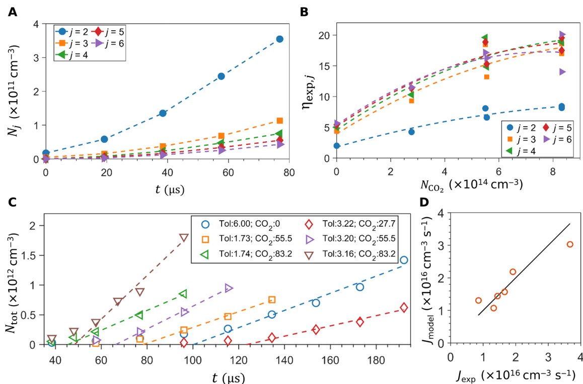
Fig. 3. Kinetic analysis of binary toluene-CO 2 nucleation at constant T_F = 55 \text{ K} and p_F = 40 \text{ Pa} . (A) Concentration N_j of the j -mers ( j = 2 to 6) as a function of the nucleation time t . The toluene and CO 2 concentrations in the postnozzle flow are 1.73 \times 10^{13} \text{ cm}^{-3} and 5.55 \times 10^{14} \text{ cm}^{-3} (CT4 in table S1), respectively. (B) Enhancement factor \eta_{\text{exp},j} as a function of the CO 2 concentration N_{\text{CO}_2} for j = 2 to 6. Dashed lines are quadratic fits to the data points (symbols). (C) Total number of clusters N_{\text{tot}} as a function of t for six different toluene-CO 2 concentrations (CT0 to CT5; table S1). The legend shows the concentrations in units of 10^{13} \text{ cm}^{-3} . The dashed lines are linear fits to the experimental data points (symbols). (D) Circles: Comparison of the experimental nucleation rates J_{\text{exp}} and the modeled nucleation rates J_{\text{model}} (Eq. 2). The straight black line is a reference line with a slope of 1.
