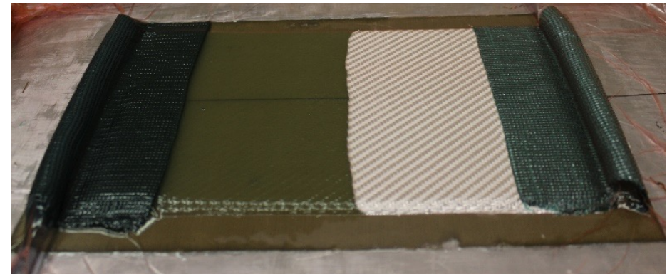
Vacuum Infusion: RTM variant
