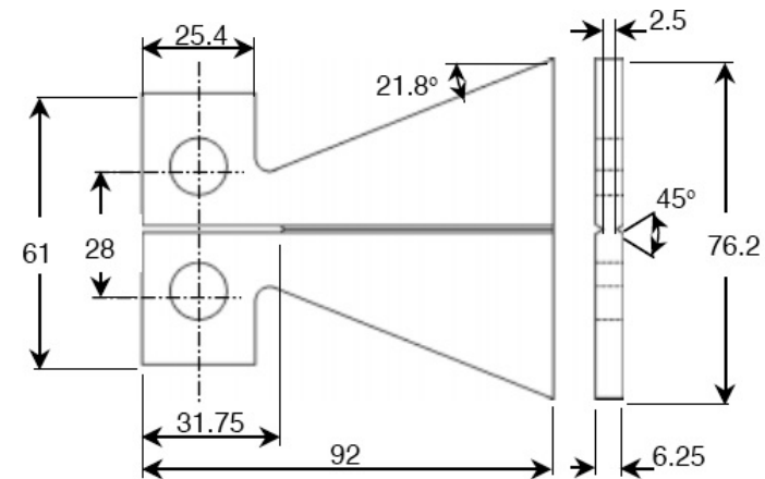
Fig. 3—Tapered double-cantilever beam (TDCB) geometry (dimensions in mm)
