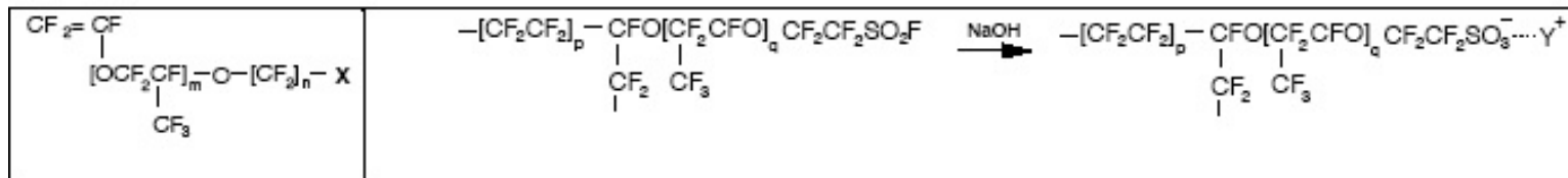
Fig. 1. The monomer (left) and the synthesis of Nafion™ (right). Note that \text{X} = \text{SO}_3^- or \text{COO}^- , m = 0-2 , n = 1-4 , p = 5-11 , and q = 1 .
