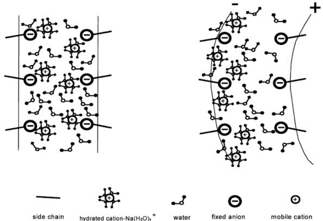
Fig. 10. Schematics of the electrophoretic migration of counter ions within IPMC network.
