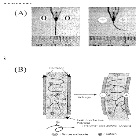
Fig.1 (A) Photograph of the bending motion of the Flemion®/gold composite driven by 2V voltage in water. (B) Schematic representation of the electromechanical model of the IPMC based on the stress due to electro-osmotic flow.
