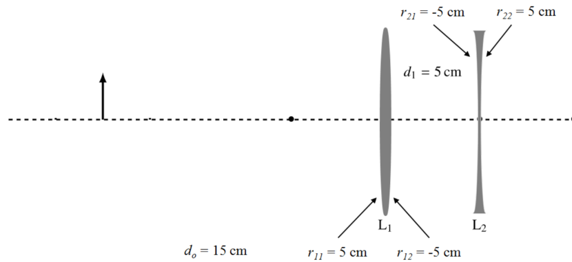
Figure 1: Two thin lenses
