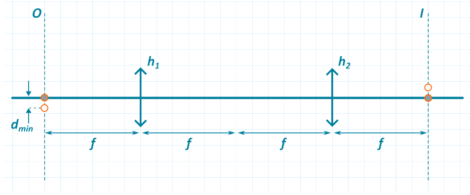
Figure 2: The 4f scheme consisting of two thin lenses. Two monochromatic sources in the object planes radiate at wavelength \lambda = 600 nm. Note: the distance between the sources d_{min} is drawn not up to scale.
