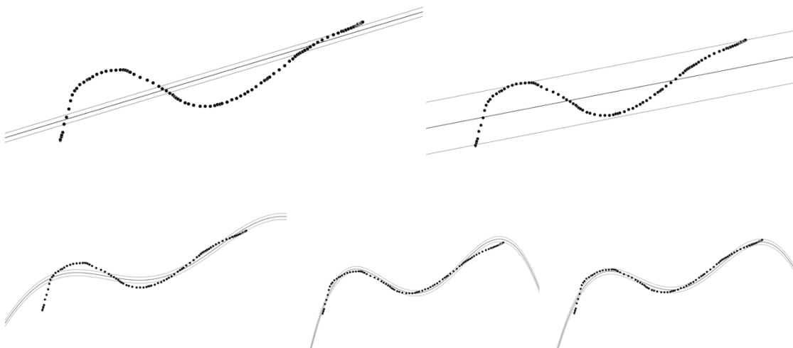
Figure 5-12: Example of \epsilon -SVR on a two-dimensional datasets. Datapoints are shown in plain dot. The regression signal is in solid line. The boundaries around the \epsilon -insensitive tube are drawn in light grey lines. using a linear kernel (top) and a Gaussian kernel (bottom). TOP: effect of the increasing the \epsilon -tube with \epsilon=0.02 (left) and \epsilon=0.1 (right). BOTTOM: effect of increasing parameter C (from left to right, C=10 , 100 and 1000 ) that penalizes for poorly fit datapoints.
