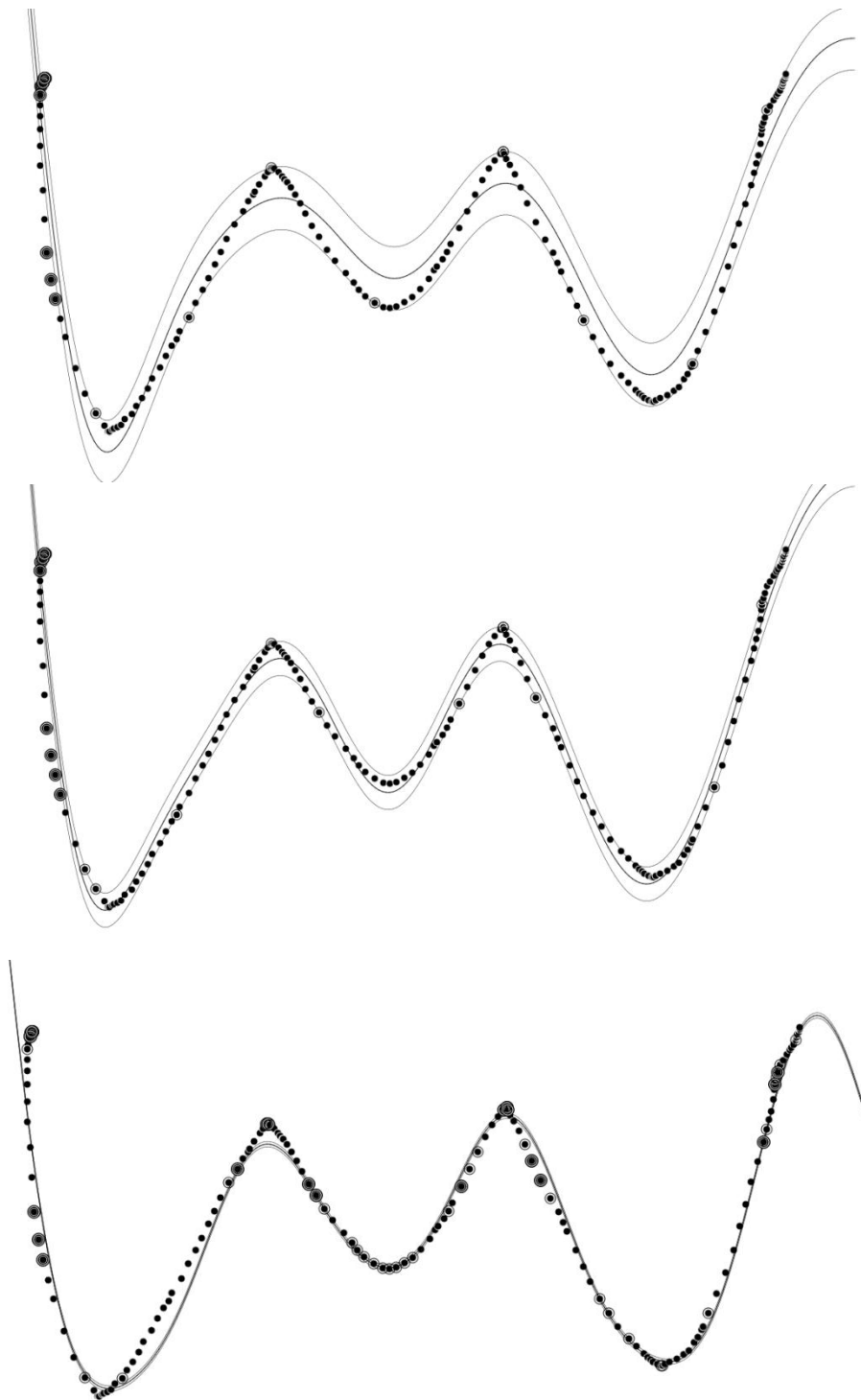
Figure 5-16: Increase of the number of support vectors and of the proportion of datapoints outside the \varepsilon -sensitive tube when increasing \nu . From top to bottom, \nu takes value 0.08, 0.1 and 0.9. \nu -SVR was fitted with C=50 and a Gaussian kernel with kernel width=0.021.
