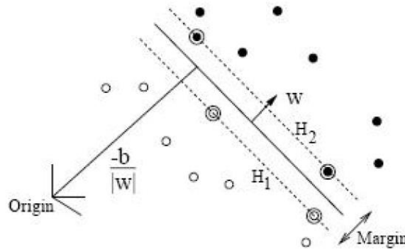
Figure 5-6: A binary classification toy problem: separate dark balls from white balls. The optimal hyperplane is shown as the solid line. The problem being separable, there exists a weight vector w and an offset b such that y^i (\langle w, x^i \rangle + b) > 0 ( i = 1, \dots, m ): Rescaling w and b such that the points closest to the hyperplane satisfy |\langle w, x^i \rangle + b| = 1 , we obtain a canonical form (w, b) of the hyperplane, satisfying y^i (\langle w, x^i \rangle + b) \geq 1 . Note that, in this case, the margin (the distance to the closest point to the hyperplane) equals 1 / \|w\| . This can be seen by considering two points x^1, x^2 on opposite sides of the margin, that is, \langle w, x^1 \rangle + b = 1, \langle w, x^2 \rangle + b = -1 , and projecting them onto the hyperplane normal vector w / \|w\| . The support vectors are the points on the margin (encircled in the drawing).
