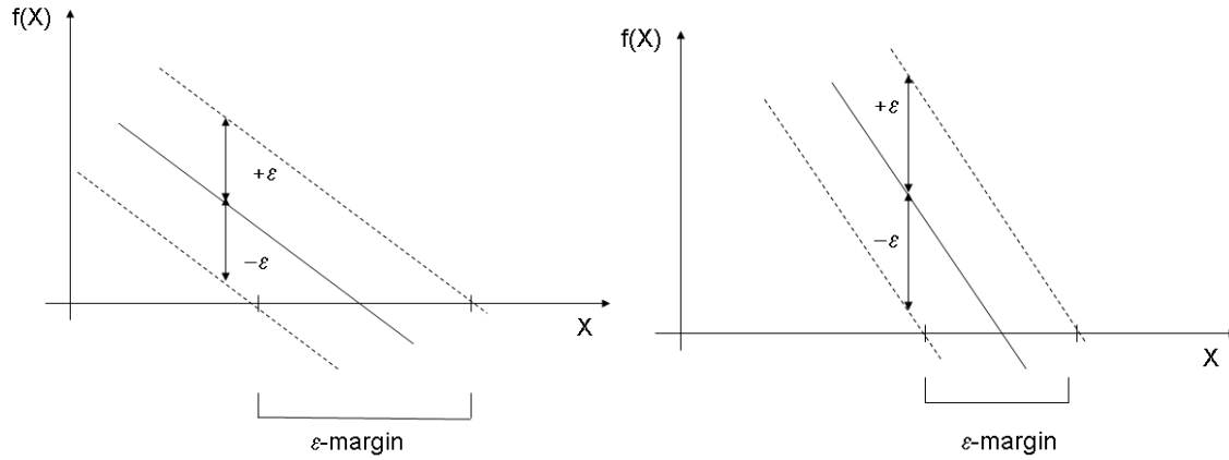
Figure 5-11: Minimizing the \varepsilon -margin in SVR is equivalent to maximizing the slope of the function f .
