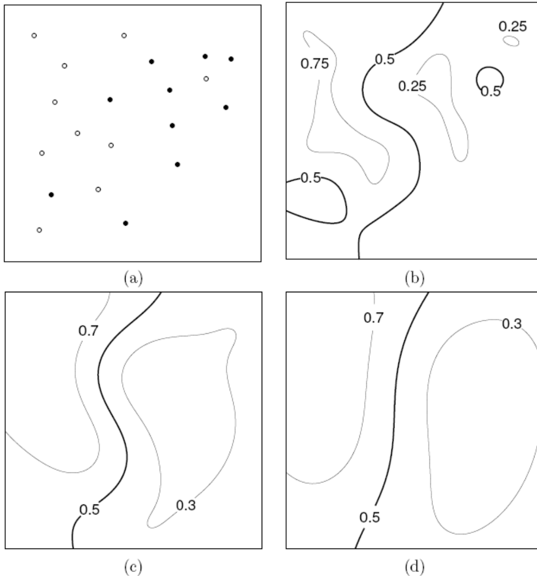
Figure 5-21: Example of successful classification with Gaussian Process classification, adapted from C. E. Rasmussen & C. K. I. Williams, Gaussian Processes for Machine Learning , the MIT Press, 2006. Panel (a) shows the location of the data points in the two-dimensional space [0, 1] . The two classes are labelled as open circles (+1) and closed circles (-1). Panels (b)-(d) show contour plots of the predictive probability \mathbb{E}[\mathbf{y}|\mathbf{x}] for signal variance \sigma^2 = 9 and length-scales \ell of 0.1, 0.2 and 0.3 respectively. The decision boundaries between the two classes are shown by the thicker black lines. The maximum value attained is 0.84, and the minimum is 0.19.
