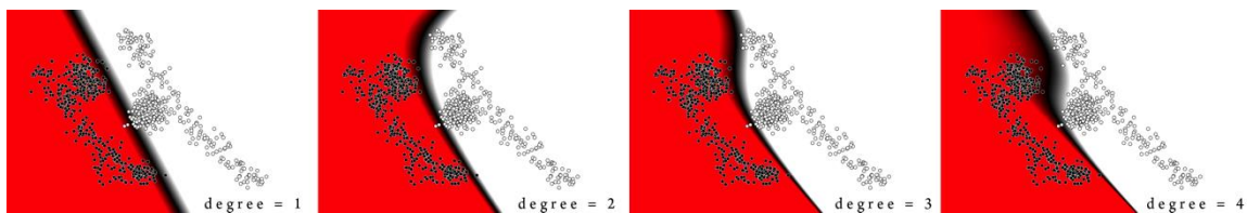
Figure 5-9: Classification using a polynomial kernel with different degrees (SVM). The data is not linearly separable (left). By increasing the degree of the polynomial, the separation plane becomes non-linear and is able to correctly separate the data. [DEMOS\CLASSIFICATION\SVM-POLY.ML]
