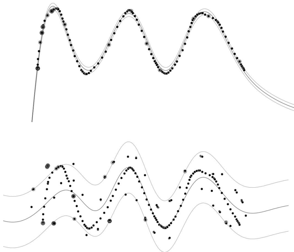
Figure 5-15: Effect of the automatic adaptation of \varepsilon using \nu -SVR. (Top) Data with no noise. (Bottom) Same dataset with a white noise. In both plots, \nu -SVR was fitted with C=100 , \nu=0.05 , and a Gaussian kernel with kernel width=0.021.
