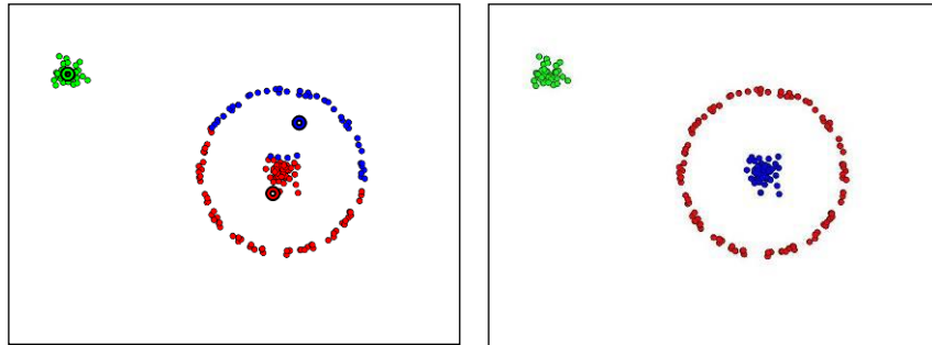
Figure 5-4: A difficult clustering problem. Standard K-Means (left) is unable to correctly separate the three clusters. Using a Gaussian kernel (gamma = 0.01) Kernel K-Means (right) successfully separates the three clusters. [DEMOS\CLUSTERING\KERNEL-KMEANS.ML]
