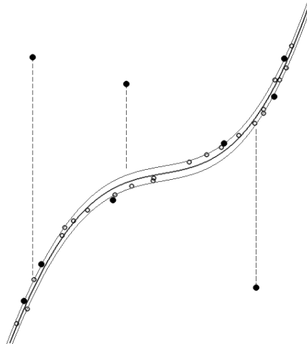
Figure 5-10: Effect of a non-linear regression through SVR. The tightness of the \square -insensitive tube around the regression signal varies along the state space as an effect of the distance in feature space between the support vectors (the support vector are plain circles). Datapoints within the \square -insensitive tube do not influence the regression model and are indicated with un-filled circles.
