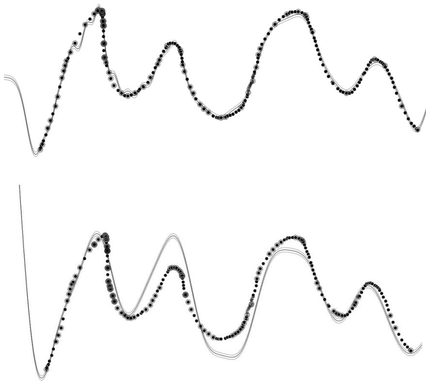
Figure 5-13: Effect of the kernel width on the fit. Here fit using C=1000 , \gamma=0.01 , kernel width=0.01 (top), 0.1 (bottom). The points encircled represent the support vectors.
