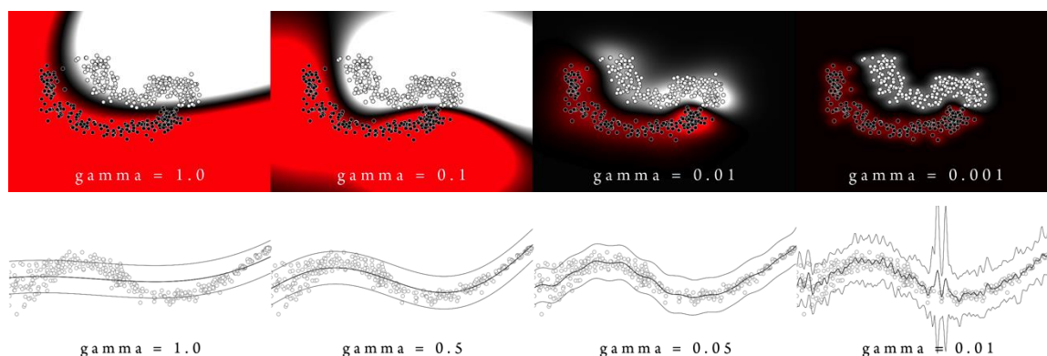
Figure 5-18: Effect of the width of a gaussian kernel on a classification task (SVM, top) and regression (GPR, bottom). When the kernel width ( \gamma ) is very small, the generalization becomes very poor (i.e. the system overfits the data and is unable to estimate correctly on samples that have never been seen). Choosing appropriate parameters for the kernel depends on the data and is one of the main challenges in kernel methods.
