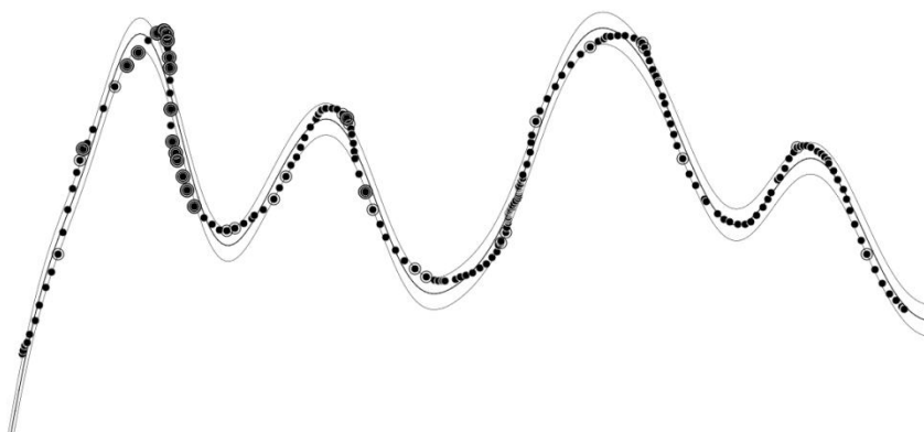
Figure 5-14: Reduction of the effect of the kernel width on the fit by choosing appropriate hyperparameters. Gaussian SVR fit using C=100 , \gamma=0.03 , kernel width=0.1.
