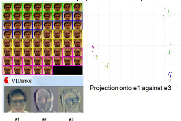
Figure 3-1: A database of images from two persons composed of 4 classes highlighted in colors is projected onto eigenvectors 1 and 3. When projecting onto e1 and e3, we can separate the image of the first person with and without glasses, as the eigenvector e3 embeds features distinctive of person1 primarily.
