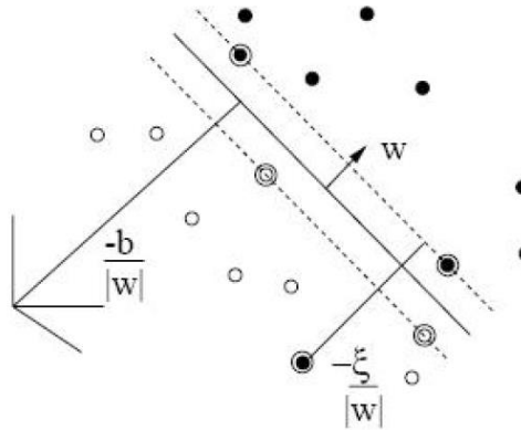
Figure 5-7: Linear separating hyperplanes for the non-separable case.
