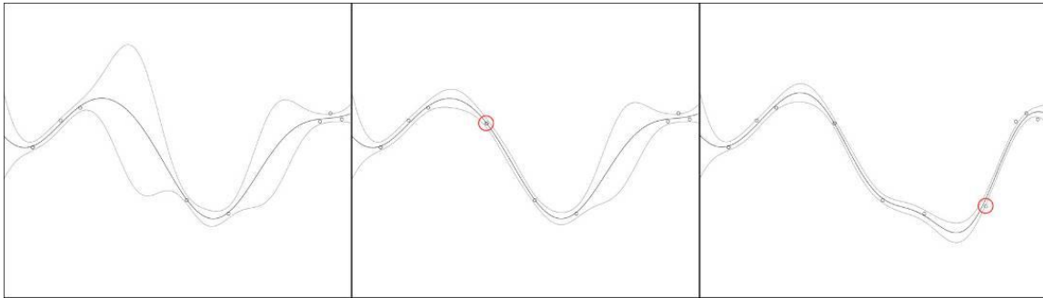
Figure 5-17: The confidence of a Gaussian Process is dependent on the amount of data present in a specific region of space (left). Regions of low data density have lower confidence. By adding points in those regions, the confidence increases (center), but the regression function will change to adapt to the new data (right).
