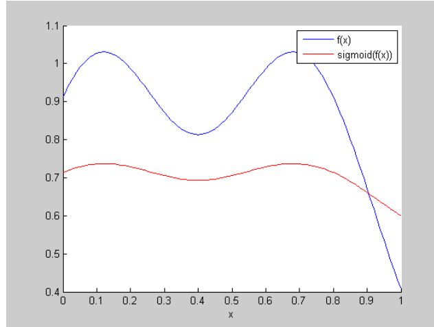
Figure 5-20: Example of an arbitrary prior function f(x) (here composed of the superposition of two Gaussian). Applying the sigmoid function on f(x) flattens the function, while normalizing between 0 and +1.
