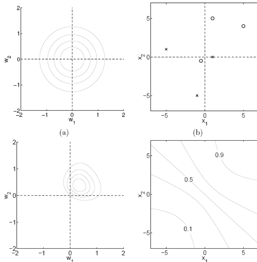
Figure 5-19: a) Contours of the prior distribution p(w) = N(0, I) . (b) dataset, with circles indicating class +1 and crosses denoting class -1. (c) contours of the posterior distribution p(w|D) . (d) contours of the predictive distribution p(y_+ = +1 | x_-) , adapted from C. E. Rasmussen & C. K. I. Williams, Gaussian Processes for Machine Learning , the MIT Press, 2006.
