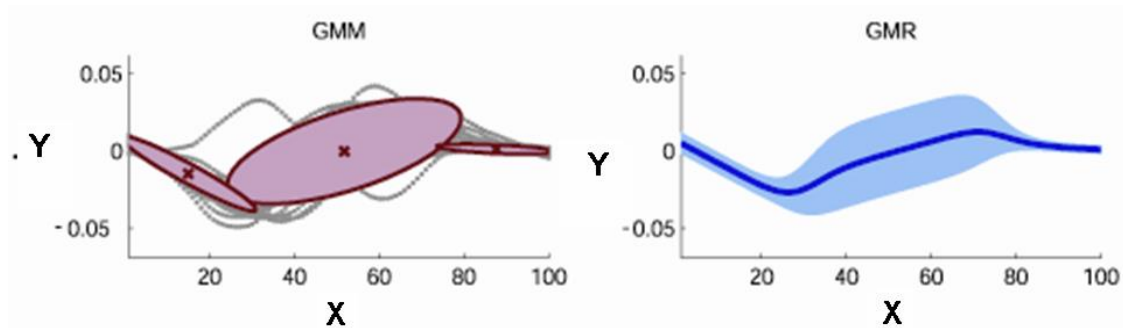
Figure 4-1: Two-dimensional illustration of a) left: a Gaussian Mixture Model with 3 Gaussians (in violet) superposed to the original set of pairs (x, y) of datapoints (in grey), b) the Gaussian Mixture Regression model resulting from the GMM. The dark line is the regression signal, i.e. E\{p(Y|X)\} . The blue envelope around it is one standard deviation computed from \text{var}\{p(Y|X)\} .
