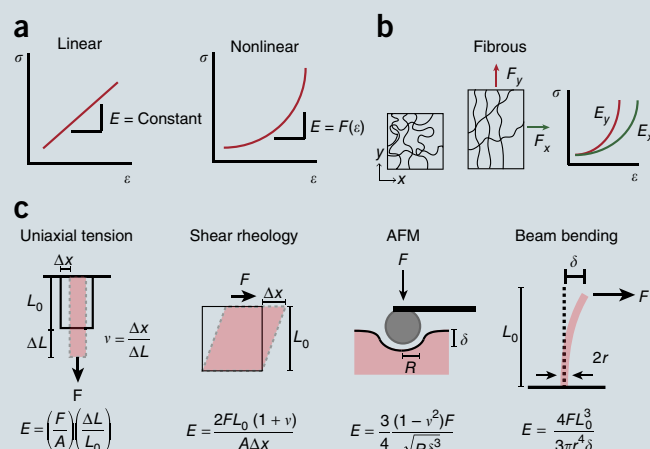
Figure 1 | ECM mechanical properties determine the relationship between force and deformation. (a) The elasticity, given here as the Young's modulus ( E ), determines the relationship between stress and strain in linear materials. In nonlinear materials, E is a function of strain. (b) The ECM is fibrous with anisotropic and nonlinear material properties. (c) Common methods for determining the mechanical properties of materials used to measure cellular forces. \nu , Poisson ratio; F , force; A , cross-sectional area. All other variables not defined in the text are geometric parameters defined as in the schematics.
