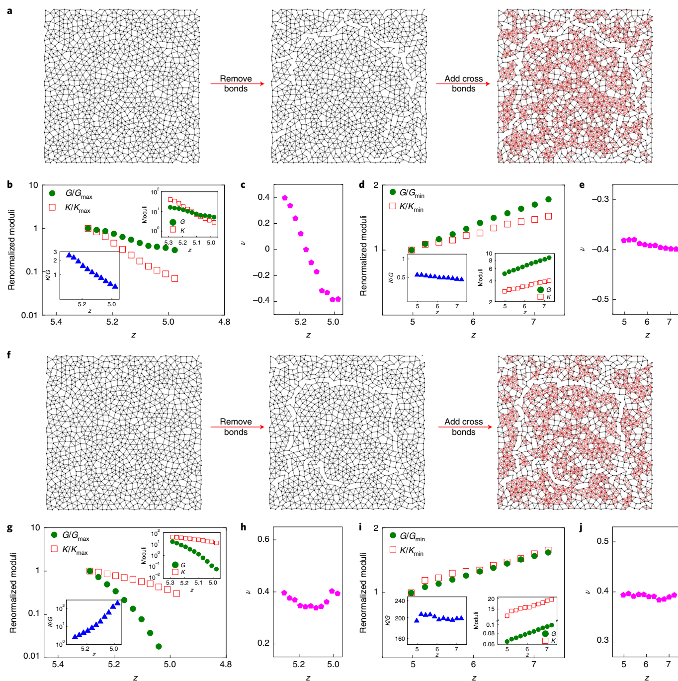
Fig. 3 | The numerical design of a network with both affine and non-affine tunability. a , The original network with z = 5.28 (left-hand panel); achieving non-affine tunability by removing the bonds important to K (middle panel); realizing affine tunability by adding the red cross bonds (right-hand panel). b , With the non-affine operation of bond removal, K reduces substantially while G changes more gently (note that the z axis decreases with this operation). Interestingly, K/G can decrease even below unity to reach the unusual situation of K < G (insets). c , \nu is also broadly tunable from positive to negative by this operation. d , With the affine operation of cross-bond addition, both K and G increase but K/G remains roughly constant (note that the z axis increases with this operation). e , \nu also stays constant under this affine operation. f , Operations similar to a except that the bonds important to G are now removed and then the cross bonds are added. g , When the bonds important to G are removed, G reduces by two orders while K remains relatively stable. Correspondingly, K/G increases substantially. h , \nu does not change much with bond removal. i, j , The affine operation of cross bond addition changes K and G simultaneously, while K/G ( i ) and \nu ( j ) remain unchanged as expected.
