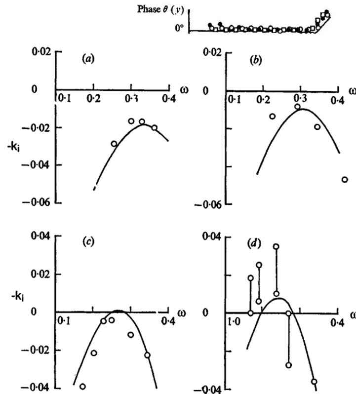
Fig. 8.5. Spatial amplification rates -k_i versus frequency \omega (Nishioka et al. , 1975). —: Itoh's theoretical prediction (1974); \circ : experiments. (a): Re = 3,000 . (b): Re = 4,000 . (c): Re = 6,000 ; experiments: Re = 5,700 . (d): Re = 8,000 ;
