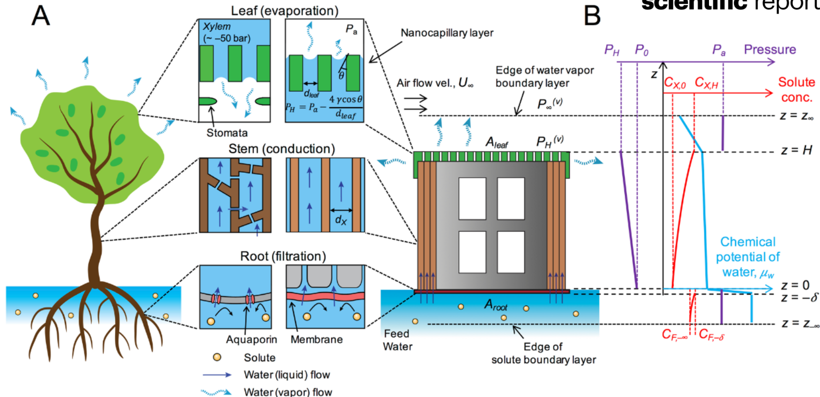
Figure 1. Overview of dewatering process by an artificial tree. (A) Schematic illustrations of a natural mangrove tree and an artificial tree for dewatering process, and their similarities in functions: filtration (root), conduction (stem), and evaporation (leaf) of water. (B) Distributions of chemical potential of water, pressure, and solute concentration through the artificial tree at different locations.
