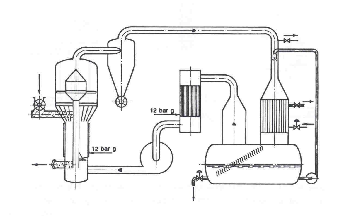
Figure 4. The pilot plant.
