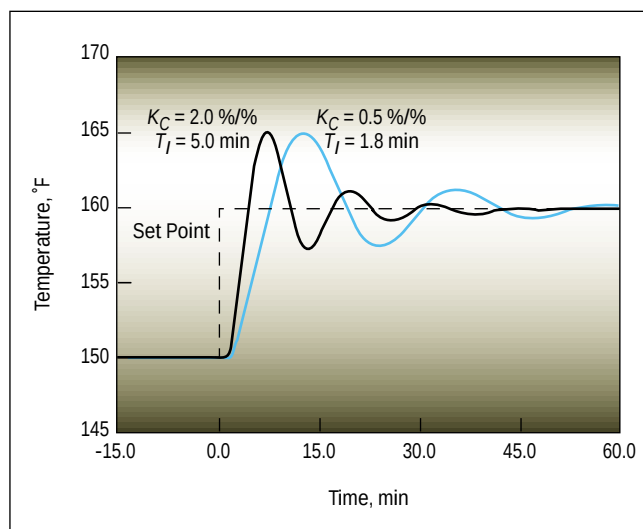
■ Figure 4. Many combinations of coefficients give quarter decay ratio.
