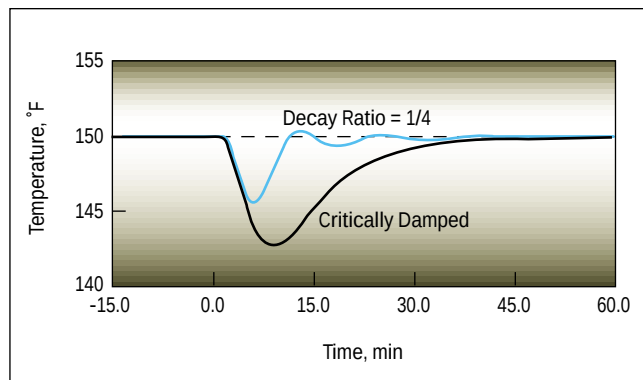
■ Figure 3. Quarter decay ratio provides better response.
