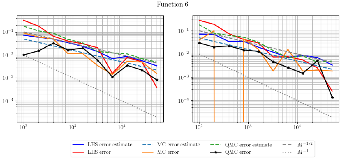
Figure 6: Function no. 6, d = 2 (left) and d = 20 (right). We remark that this is a nasty function to estimate.
