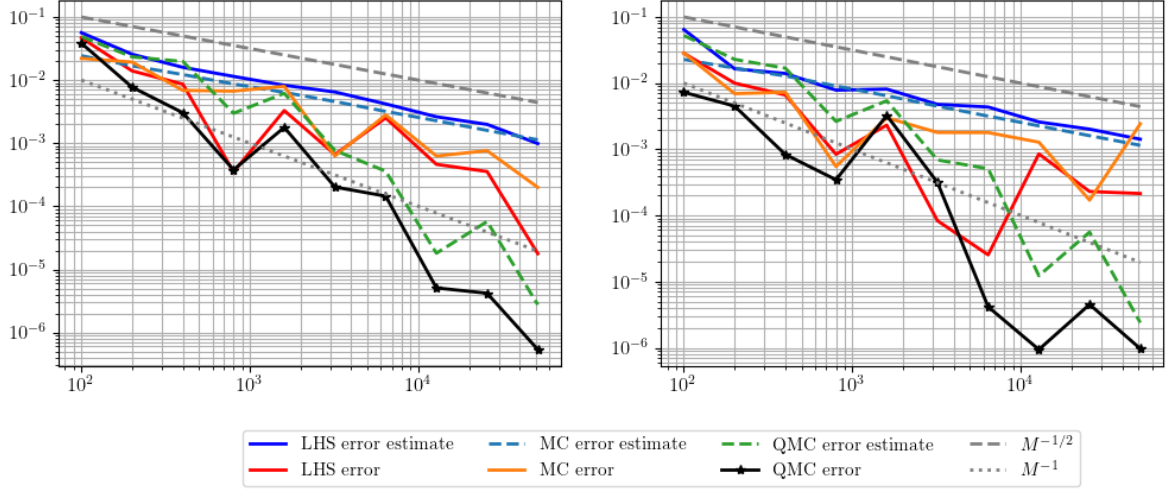
Figure 3: Function no. 3, d = 2 (left) and d = 20 (right)
