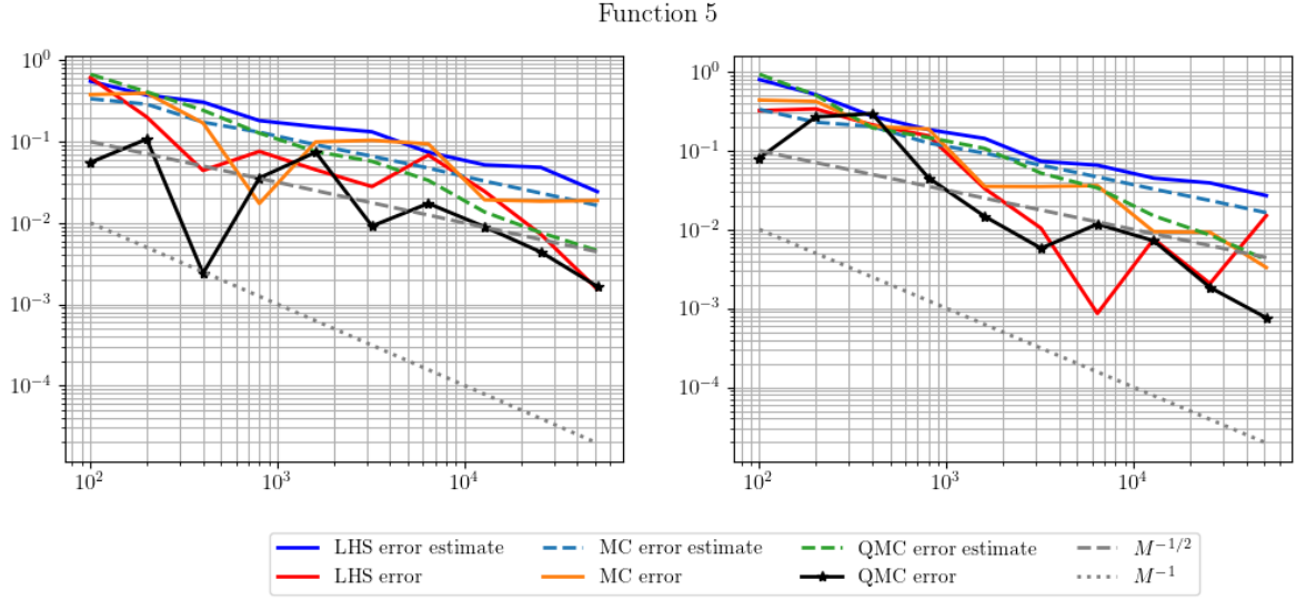
Figure 5: Function no. 5, d = 2 (left) and d = 20 (right)
