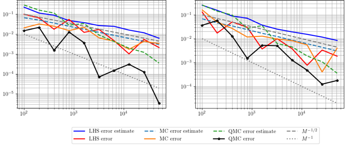
Figure 1: Function no. 1, d = 2 (left) and d = 20 (right)
