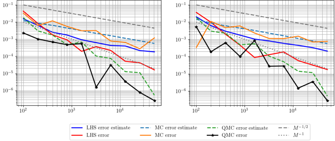
Figure 4: Function no. 4, d = 2 (left) and d = 20 (right)
