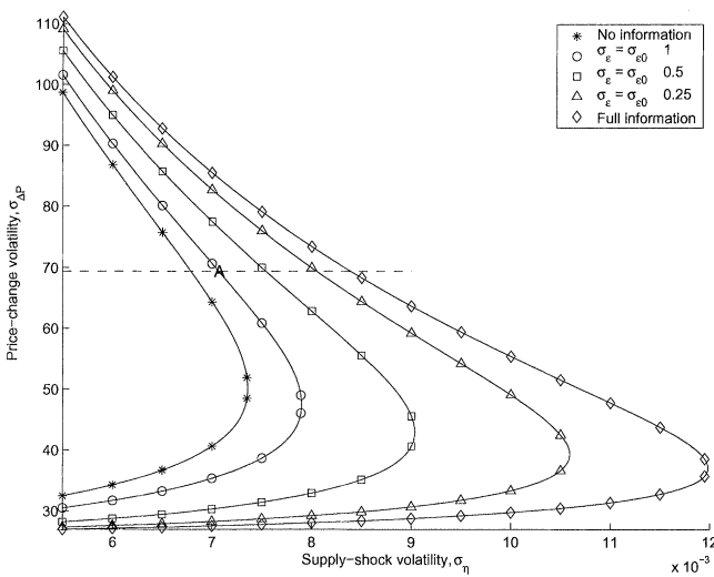
Figure 3. Volatility of the price change in a single-security model. The dashed line corresponds to Shiller's (1981b) aggregate volatility estimate, 69.4. Point A gives this volatility level under \sigma_\varepsilon = \sigma_{\varepsilon 0} \equiv 62.2 . Parameter values: \sigma_\delta = 16.5 , \Sigma_\zeta^{1/2} = 4\sigma_\eta , and r = 5\% per annum or 1.05^{10} - 1 .
