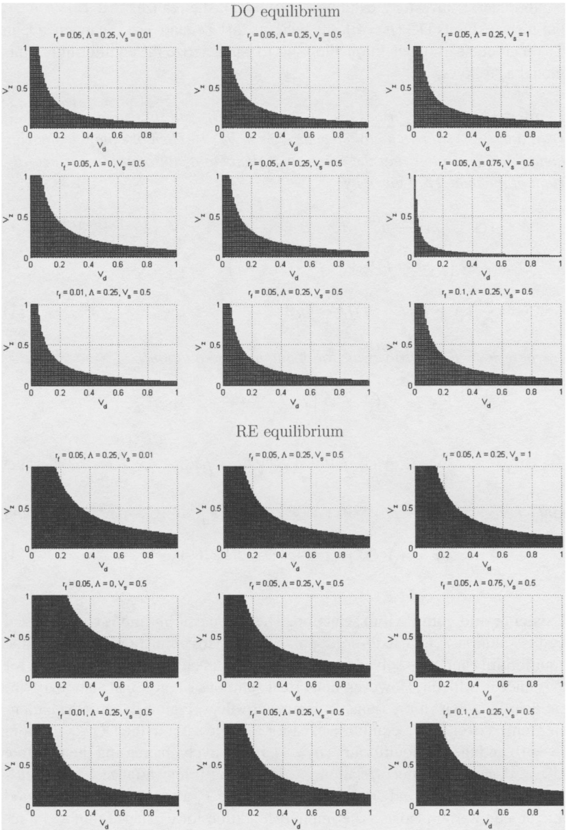
Figure 1 Existence of stationary equilibria
