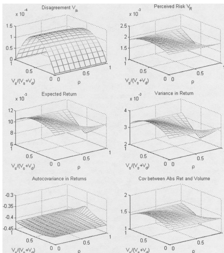
Figure 7 Model predictions in high-volatility equilibrium
