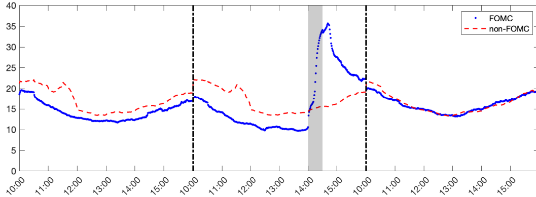
Figure 2: Realized Volatility
