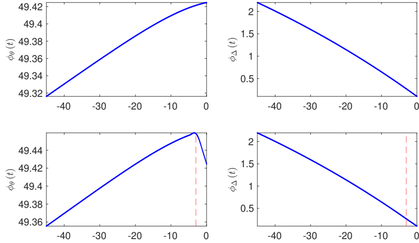
Figure 9: Pricing functions
