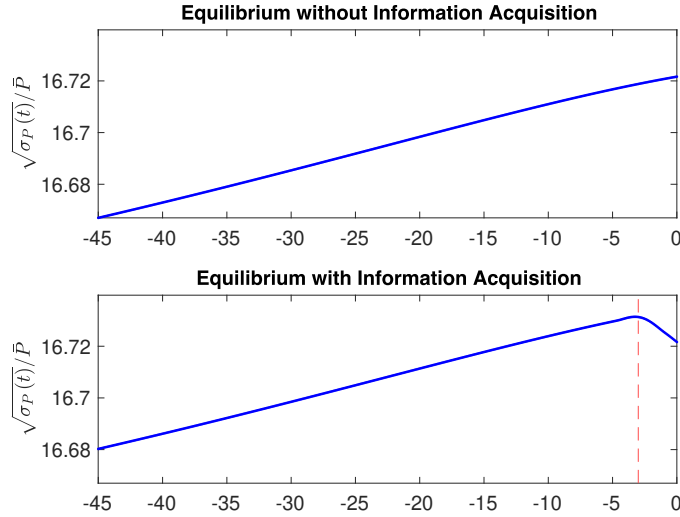
Figure 10: Realized Volatility
