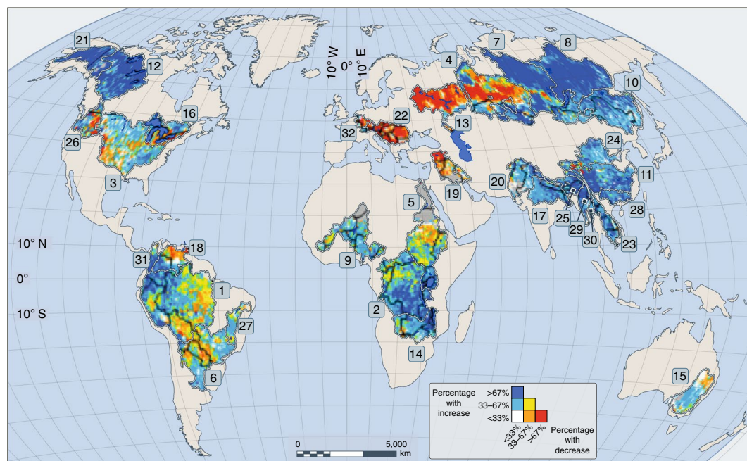
Fig. 3 | Consistency (percentage of all models) in the magnitude of estimated 100-year recurrence interval floods in 2050 from 21 climate models 75 , showing regions of increased (blue) and decreased (red) flow. Grey shaded areas are those with annual runoff <10 mm year -1 . Numbers refer to river basins listed in Fig. 1.
