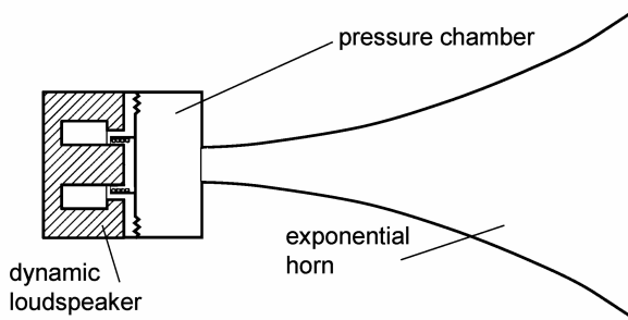
Fig. 15.14. Horn loudspeaker with pressure chamber
