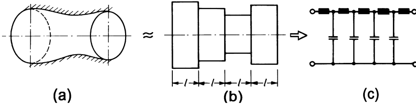
Fig. 8.10. Approximation of a tube with varied cross-sectional area
