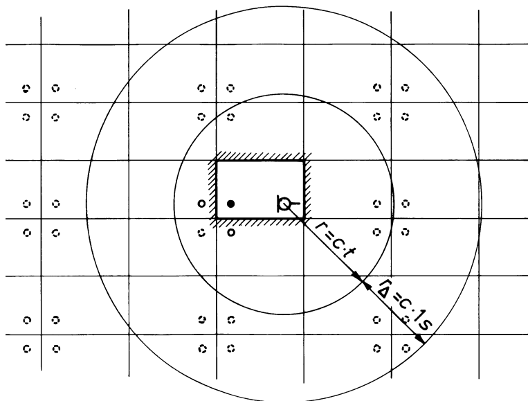
Fig. 12.9. Image sources of one sound source for a rectangular room
