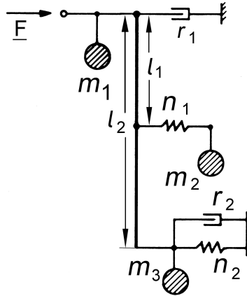
Fig. 15.3. Mechanic circuit to be converted into an equivalent electric one by analogy #2
