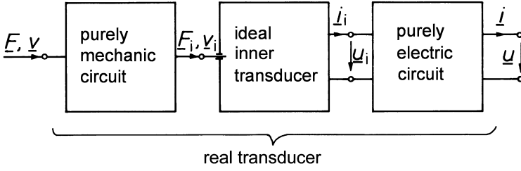
Fig. 4.5. A real transducer as a chain of three two-ports
