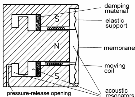
Fig. 5.10. Moving-coil microphone
