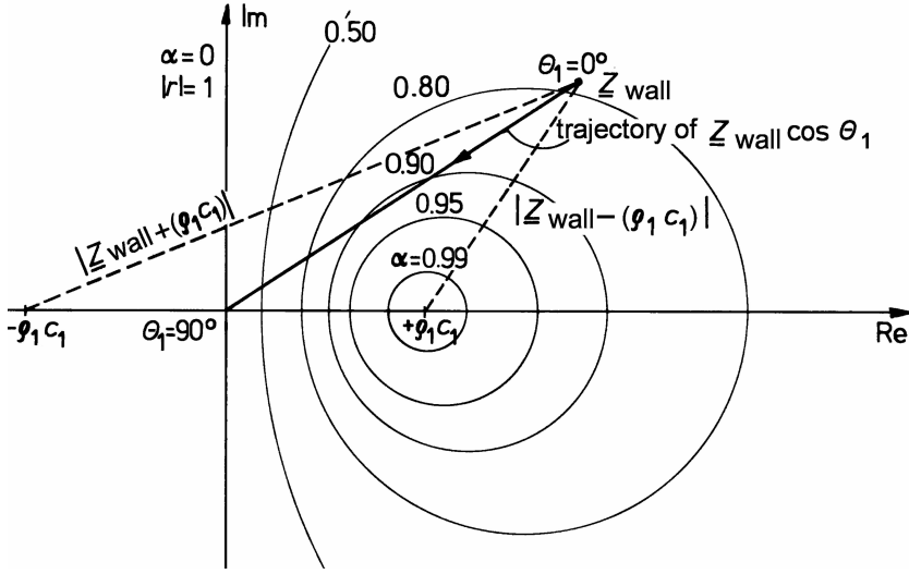
Fig. 11.6. Trajectories of constant degrees of absorption, \alpha , in the complex \underline{Z} -plane
