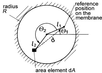
Fig. 10.9. Coordinates for calculating the radiation resistance of a circular piston
