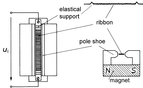
Fig. 5.9. Ribbon microphone
