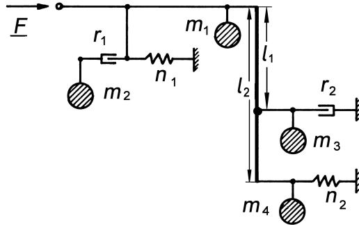
Fig. 15.4. Mechanic circuit to be converted into an equivalent electric one by analogy #1
