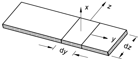
Fig. 13.4. Element of a plate with mass and bending stiffness
