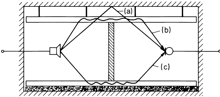
Fig. 13.12. Possible paths of sound transmission between two enclosed spaces
