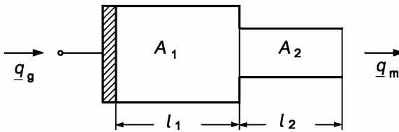
Fig. 15.15. Stepped tube composed of two sections with pressure chamber
