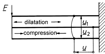
Fig. 6.5. Piezoelectric layers as a bending vibrator
