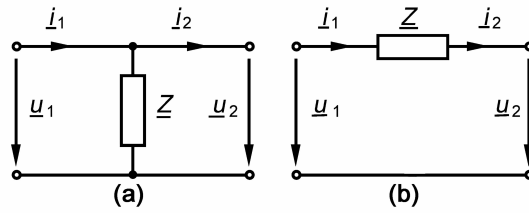
Fig. 15.8. Two-port representation of acoustic and/or electric elements
