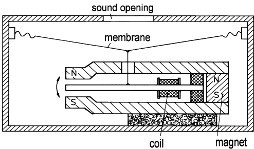
Fig. 5.14. Hearing-aid microphone
