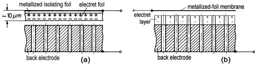
Fig. 6.20. Electret microphone, (a) version with electret membrane, (b) version with electret back electrode
