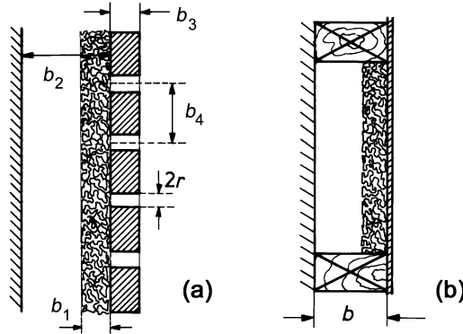
Fig. 11.13. Resonance absorbers. (a) Helmholtz absorber, (b) membrane absorber
