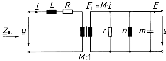
Fig. 5.3. Equivalent circuit for a magnetodynamic transducer
