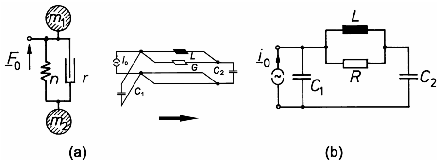
Fig. 3.8. Analogous circuit diagram (analogy # 2) of a two-mass mechanical oscillator, (a) mechanic arrangement, (b) analogous electric circuit. The plot in the middle illustrates how the electric circuit is derived
