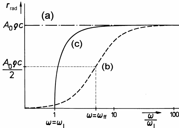
Fig. 8.6. Schematic plot of the radiation resistance of (a) a tube, (b) a conical horn, and (c) an exponential horn. Frequencies normalized to the limiting frequency, \omega_1 , of the exponential horn
