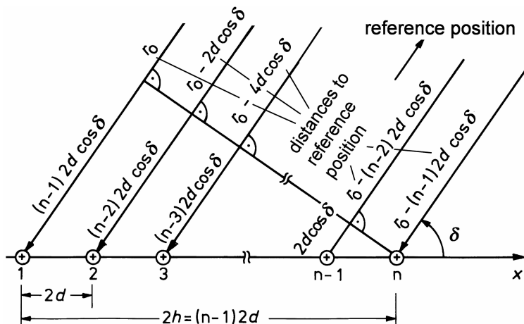
Fig. 9.6. Linear array with monopole sources
