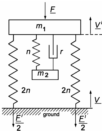
Fig. 15.18. Dynamic absorber
