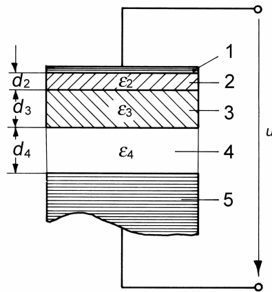
Fig. 15.11. Schematic plot of an electret microphone
