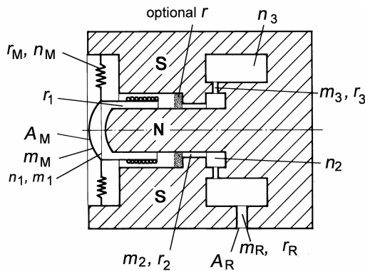
Fig. 15.10. Schematic plot of a moving-coil microphone.
