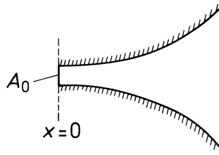
Fig. 8.5. Exponential horn
