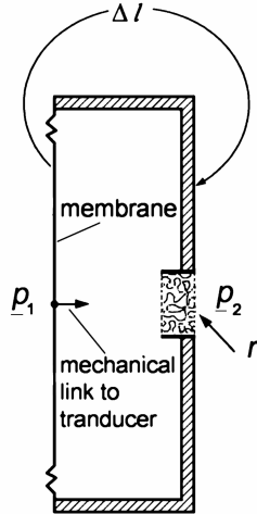
Fig. 15.9. Schematic plot of a microphone with rear opening. p_1, p_2 ... sound-pressure signals at front- and backside
