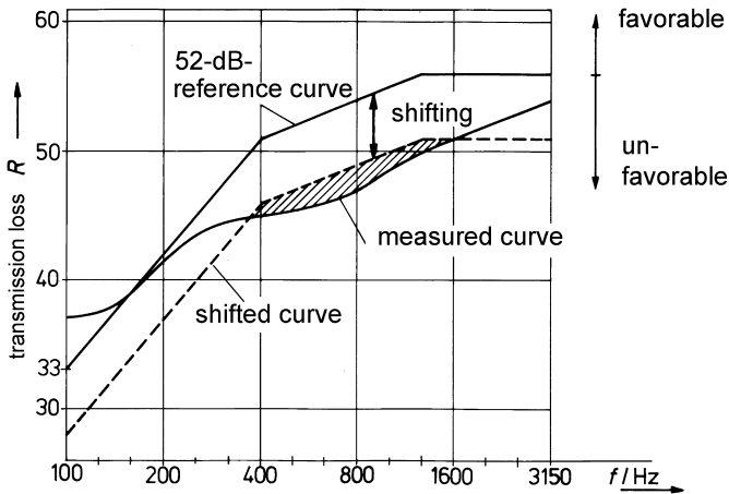
Fig. 13.13. Determination of the Weighted Sound-Reduction Index
