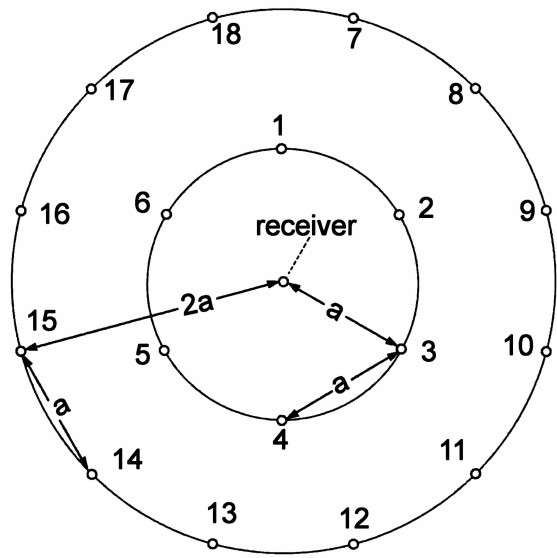
Fig. 15.2. Multiple sound sources of equal intensity in an open-space office
