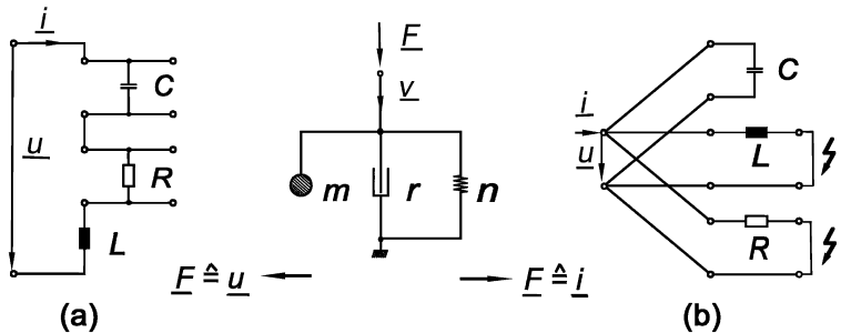
Fig. 3.6. Electric analogies of a simple mechanic parallel-branch oscillator, (a) analogy # 1, (b) analogy # 2
