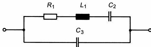
Fig. 15.12. Equivalent circuit of a quartz oscillator
