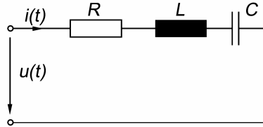
Fig. 15.1. Serial circuit of R, L and C
