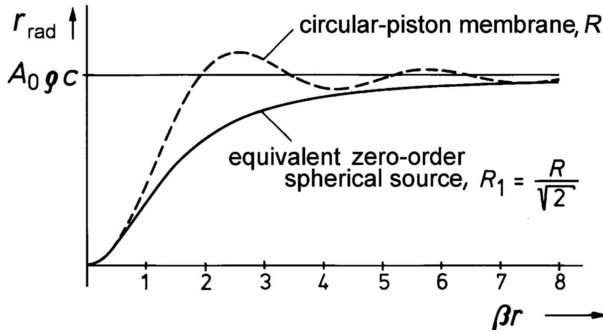
Fig. 10.10. Radiation resistance of a circular-piston membrane as a function of distance and wavelength
