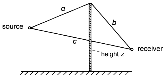
Fig. 14.9. Sound barrier
