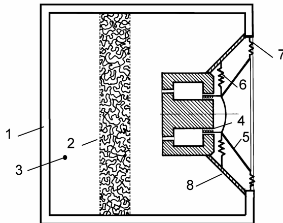
Fig. 15.7. Mechanic-acoustic circuit of a loudspeaker box to be converted into an equivalent electric one by analogy #2
