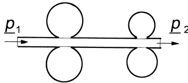
Fig. 15.6. Acoustic circuit to be converted into an equivalent electric one by appropriate analogy
