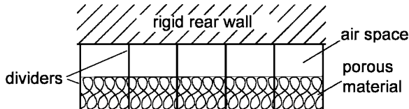
Fig. 11.11. Cassetted porous absorber
