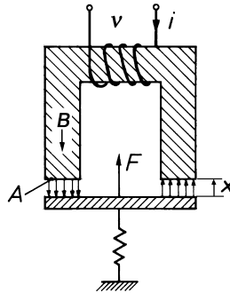
Fig. 5.12. Electromagnet with a movable armature
