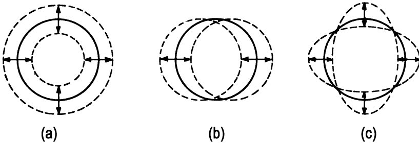
Fig. 9.2. Sound sources for spherical waves. (a) 0 th -order source, also called breathing sphere , (b) an example of 1 st -order sources, also called rigid oscillating spheres , (c) an example of 2 nd -order sources. NB: There are 2n + 1 possible modes per order, n , with n = 0, 1, 2 \dots
