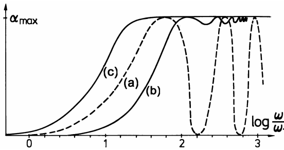
Fig. 11.10. Absorption of porous material as a function of frequency – schematic (a) finite layer with air gap, (b) finite layer directly on wall, (c) infinite thickness
