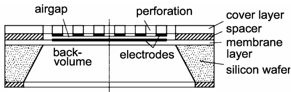
Fig. 6.19. Silicon-chip microphone (schematic)
