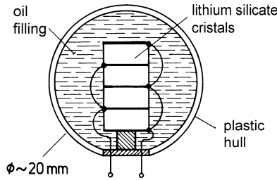
Fig. 6.7. Piezoelectric hydrophone
