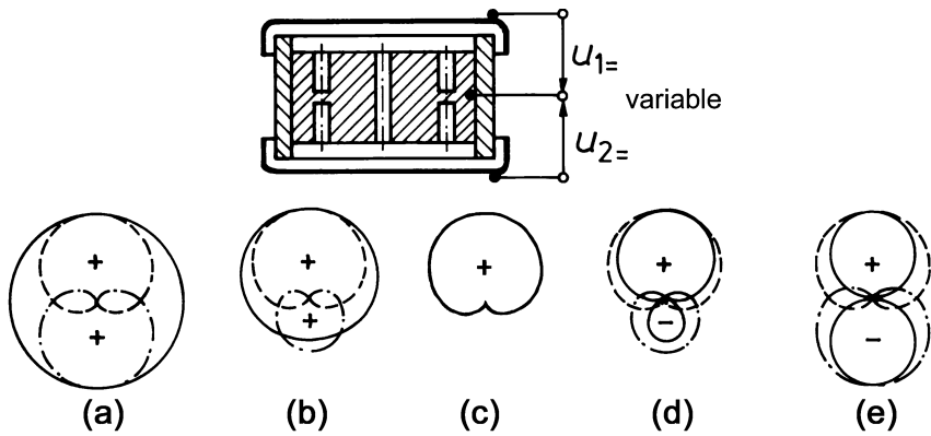
Fig. 6.18. Microphone with steerable directional characteristic, (a) sphere (b) wide-angle cardioid, (c) cardioid (d) super cardioid, (e) figure-of-eight
