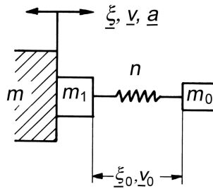
Fig. 15.5. Two-mass arrangement for vibration measurements
