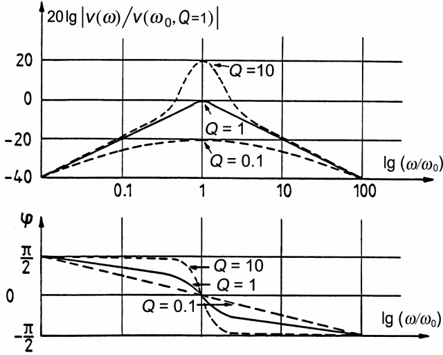
Fig. 2.6. Double-logarithmic plot of resonance curves of the particle velocity, illustrating the role of the sharpness-of-resonance factor, Q
