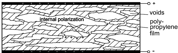
Fig. 6.21. Piezoelectret film
