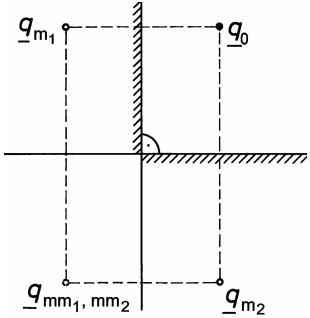
Fig. 12.5. Mirror sources at edges and in corners
