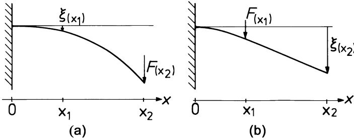
Fig. 4.8. Mechanics reciprocity experiment with a bending beam, (a) Force applied at position x_2 , deflection at position x_1 , (b) vice versa
