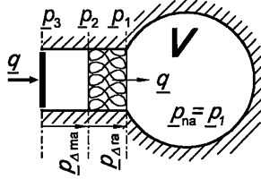
Fig. 2.8. Helmholtz resonator with friction
