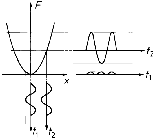
Fig. 5.1. Linearization of force characteristics
