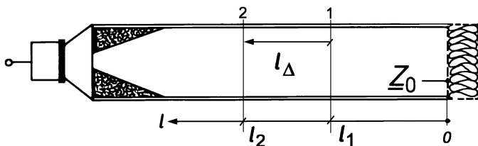
Fig. 7.8. Impedance measurement with the transfer-function method
