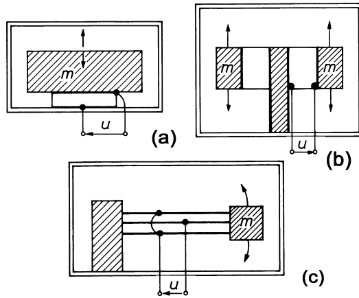
Fig. 6.8. Acceleration/velocity sensors
