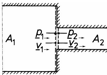
Fig. 8.7. Tube with steps in the area function
