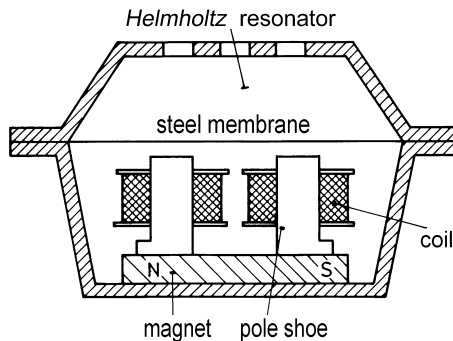
Fig. 5.13. Telephone-receiver capsule
