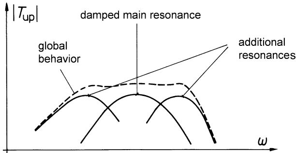
Fig. 5.11. Mechanic tuning of a moving-coil microphone
