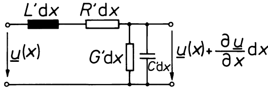
Fig. 11.1. Equivalent circuit for spatially-damped plane-wave propagation
