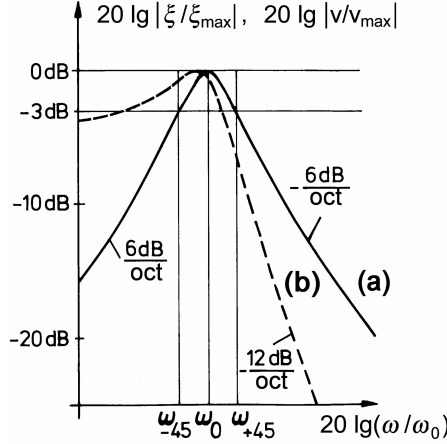
Fig. 2.5. Mechanic responses as a function of frequency for constant-amplitude forced excitation, (a) velocity, (b) elongation
