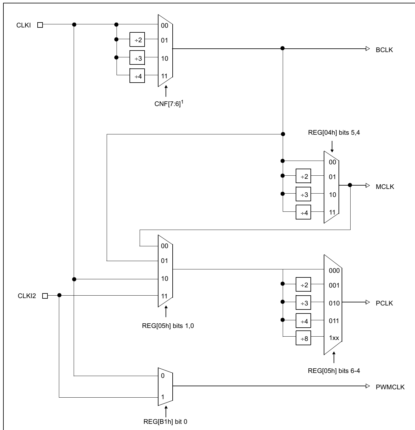
Figure 7-1: Clock Selection
