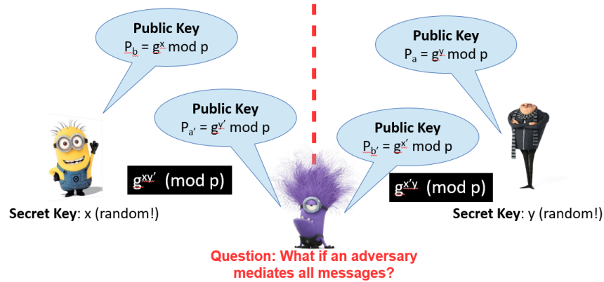
Figure 4: Diffie Hellman key exchange interception.
