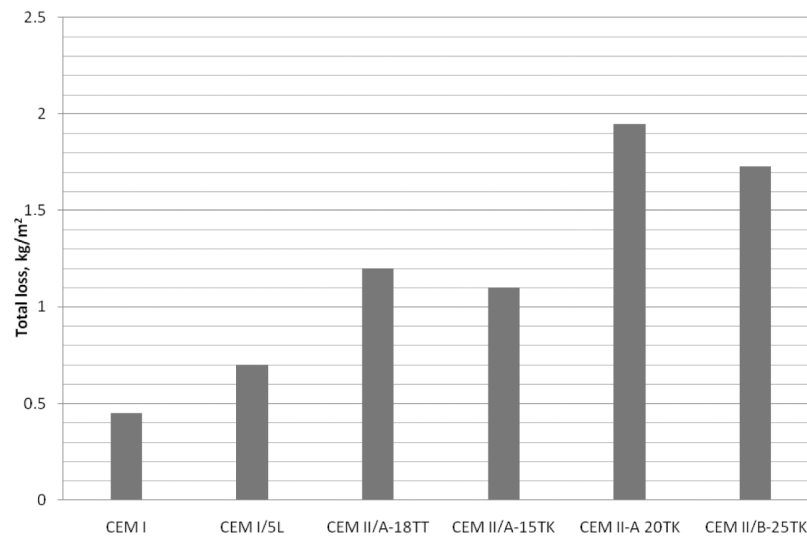
Fig. 3. Total loss of the scaled material from the surface of concrete after 56 freeze-thaw cycles in distilled water. Concretes made with Portland cement ( 320 \text{ kg/m}^3 ) using limestone as a coarse aggregate.
