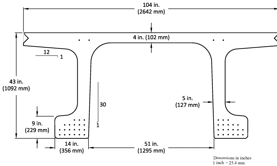
Figure 3. Strand layout of 43-inch (1,092.2-mm)-deep section for 105-ft (32.0-m)-span.
