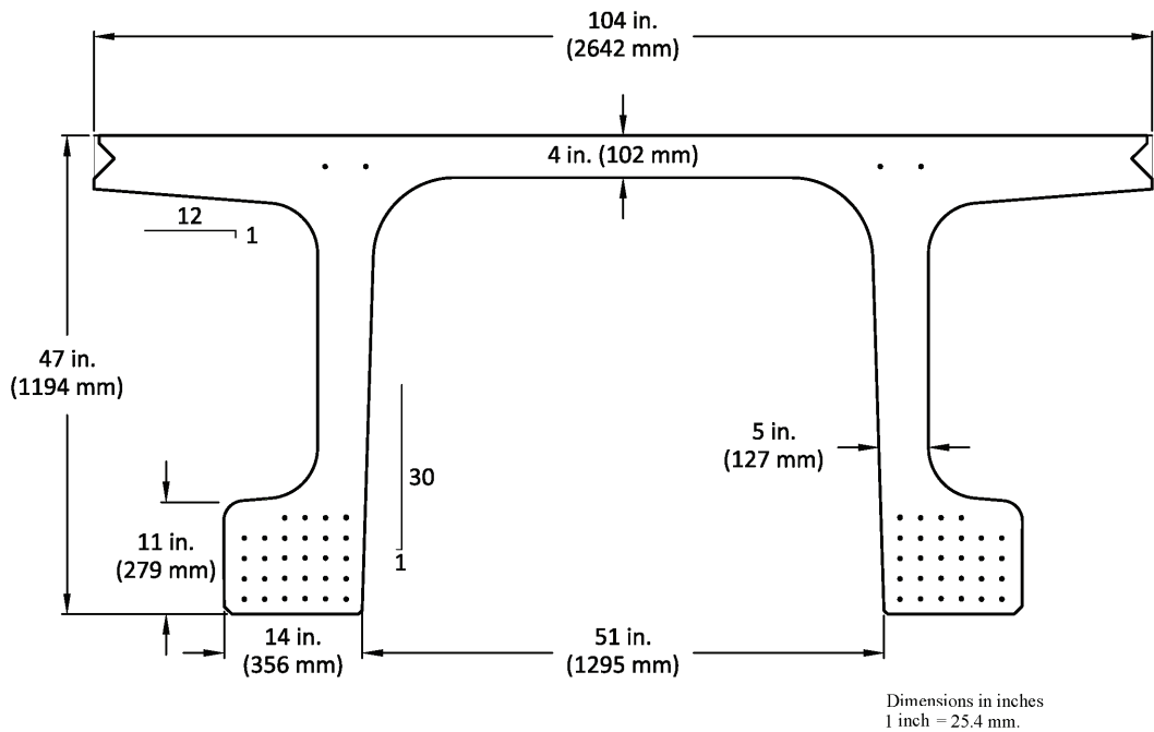
Figure 4. Strand layout of 47-inch (1,193.8-mm)-deep section for 135-ft (41.1-m)-span.
