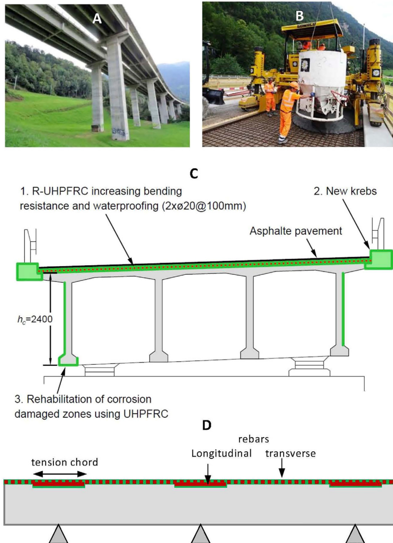
FIGURE 10 | Rehabilitation of the Arth-Goldnau Viaducts. (A) Photograph the first twin viaducts (Photograph: E. Brühwiler), (B) UHPFRC casting (Photograph: A. Weykeystone), (C) , (D) schemes of the interventions.
