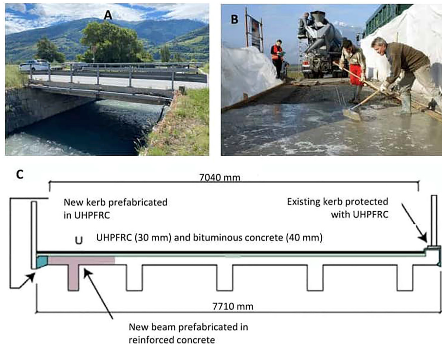
FIGURE 6 | Bridge over La Morge river. (A) Photograph of the bridge 18 years after the intervention (Photo N. Bertola); (B) UHPFRC pouring (Photo A. Hertzog); (C) scheme of the intervention using UHPFRC.
