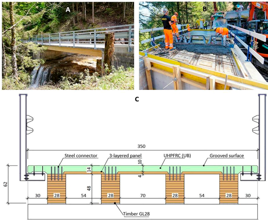
FIGURE 15 | Fruttli Bridge. (A) Photograph of the bridge; (B) pouring of the UHPFRC deck. (C) section of the composite timber-UHPFRC bridge. (Photographs: E. Kälin).
