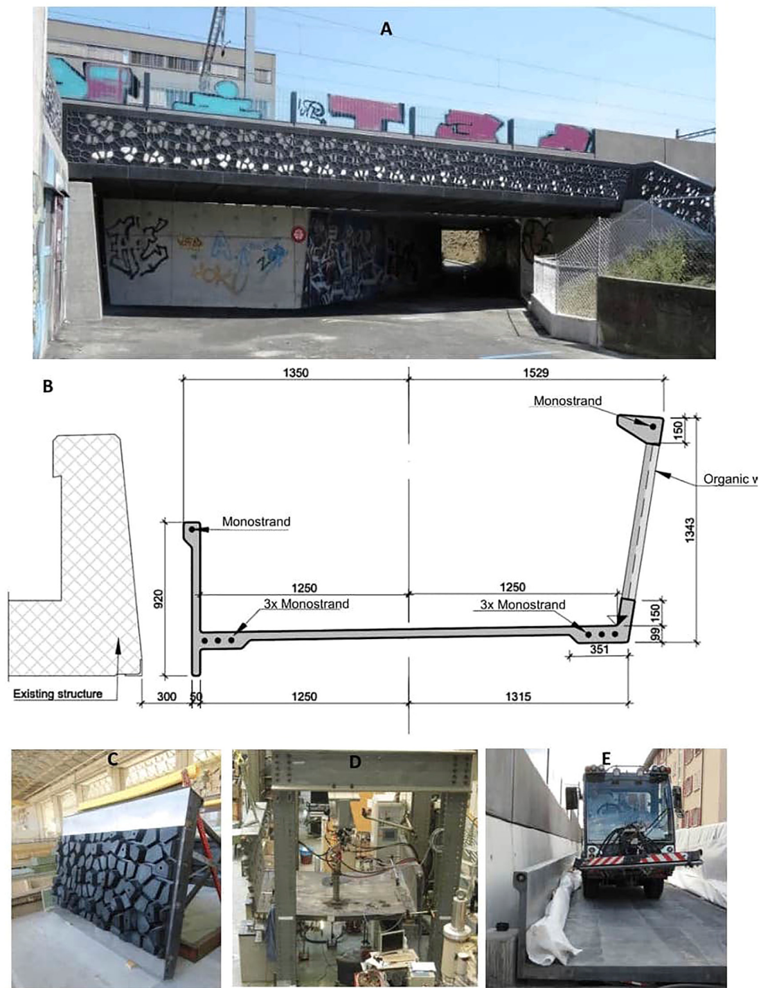
FIGURE 11 | Martinet footbridge. (A) Photograph of the footbridge; (B) Drawing of section. (C) Mold for the organic web of the Martinet footbridge; (D) laboratory test on the deck; (E) in-situ load test. (Photographs: E. Brühwiler).
