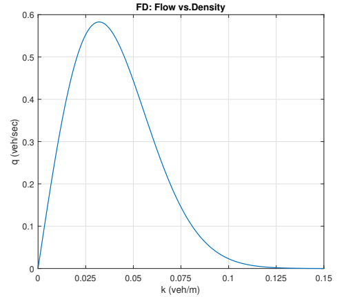
Figure 1: The Drake's Fundamental Diagram between flow and density (see Equation 9) for the case of question d, where \alpha = 10.96 and q_{crit} = 0.583 veh/sec = 2100 veh/h.
