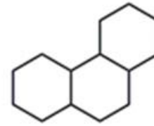
Active Molecule
