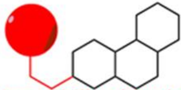
Immobilized Probe
