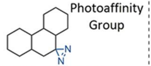
Photoaffinity Probe
