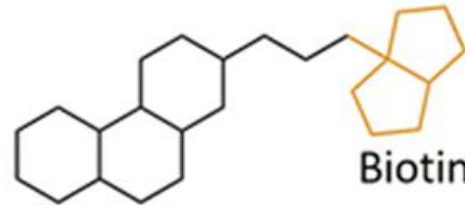
Activity-based Probe
