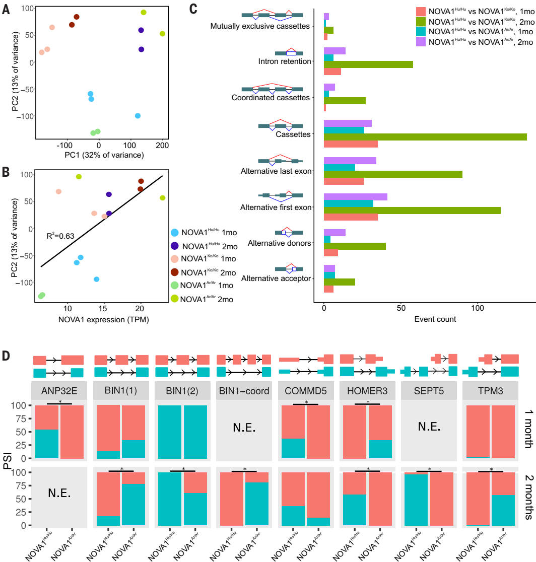
Fig. 4. Global analysis of splicing among different samples. (A) A plot of the first two principal components from a PCA of cassette inclusion frequency shows that replicates from different cell lines cluster together. Note how NOVA1 Ko/Ko cluster differently from the other edited versions. (B) The second principal component positively correlates with NOVA1 expression. (C) Numbers of differential splicing events of different types from comparisons between NOVA1 Hu/Hu and NOVA1 Ar/Ar cortical organoids at early and late stages of maturation. More differential splicing is found between NOVA1 Hu/Hu and NOVA1 Ko/Ko than between NOVA1 Hu/Hu and NOVA1 Ar/Ar , and more differential splicing is found at later stages than at early stages. (D) A set of genes exhibiting alternative splicing changes on the basis of NOVA1 variants at different stages of maturation. N.E. (not expressed) refers to splicing events with insufficient expression for splicing analysis.
