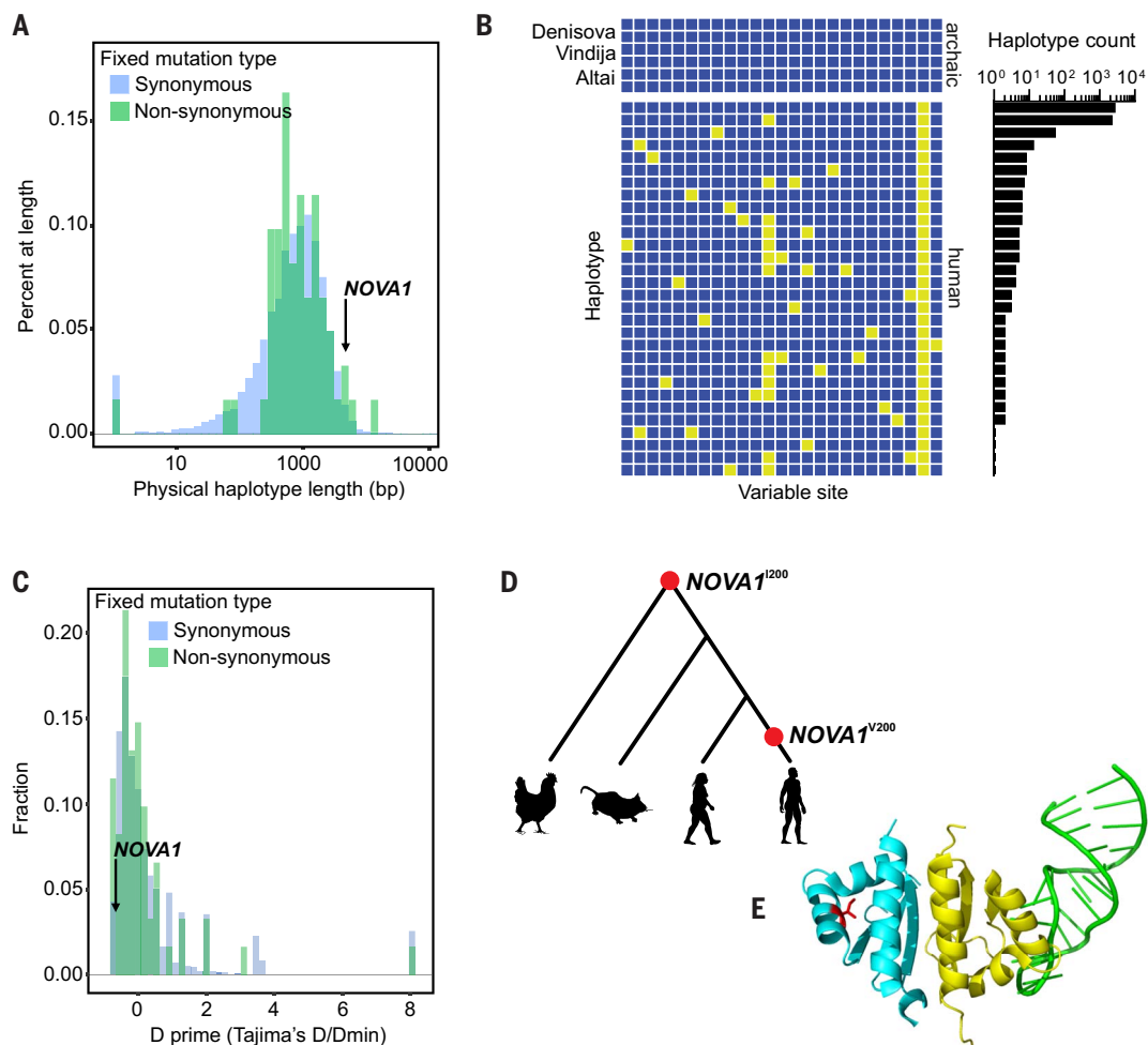
Fig. 1. Catalog of human versus Neanderthal genetic variation and the NOVA1 haplotype.
