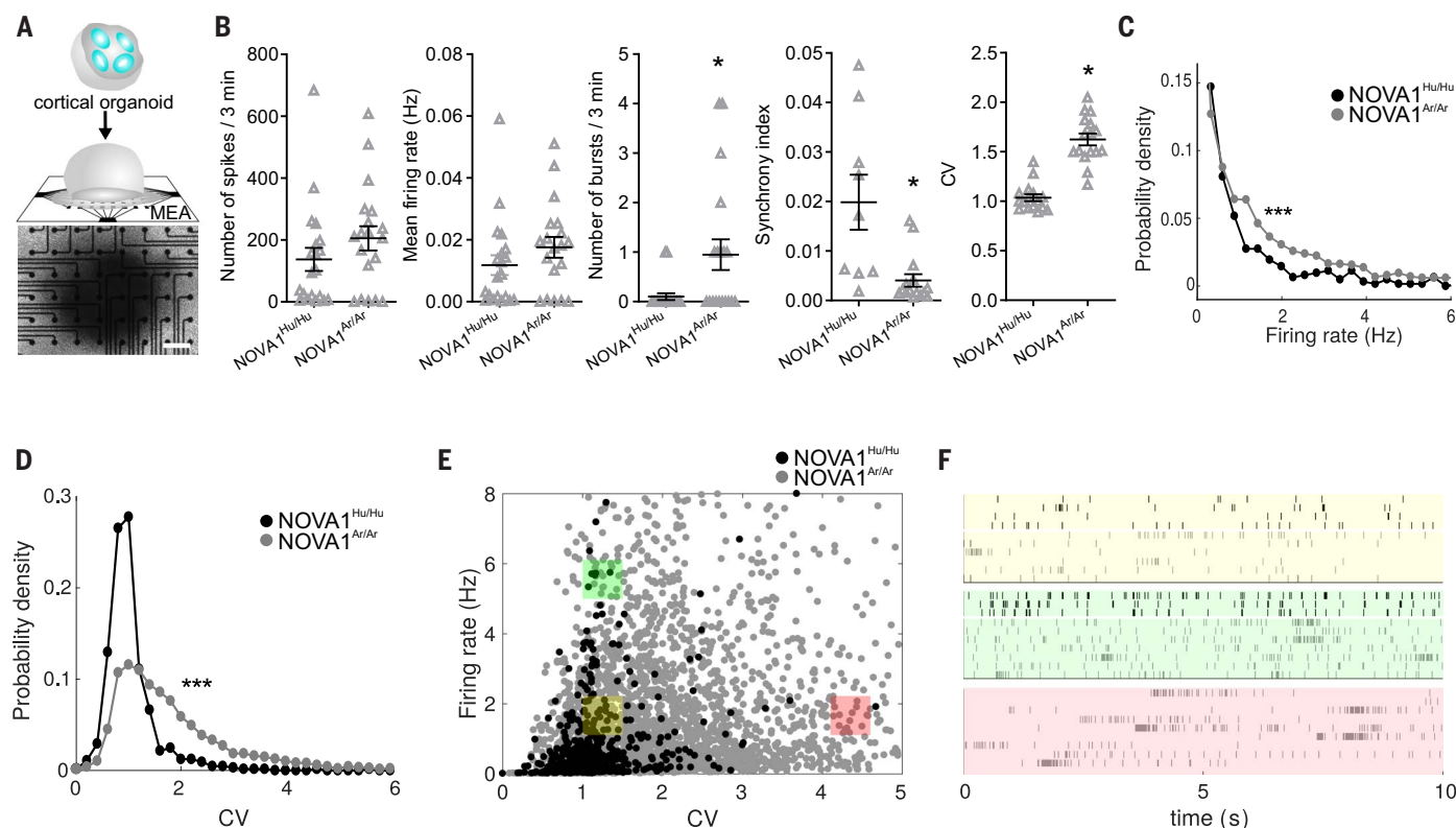
Fig. 7. Introduction of NOVA1 archaic genetic variant in modern human alters neuronal network activity. (A) Scheme of a cortical organoid plated on a MEA. Scale bar, 200 \mu m. (B to F) MEA analyses revealed an increase in spontaneous neuronal bursts in NOVA1 Ar/Ar compared with NOVA1 Hu/Hu cortical organoids (B). Although the number of total spikes does not differ, NOVA1 Ar/Ar shows a reduced synchrony index. Data are shown as mean \pm SEM ( n = 20 MEA wells per genotype); * P < 0.05, two-sided unpaired Student's
