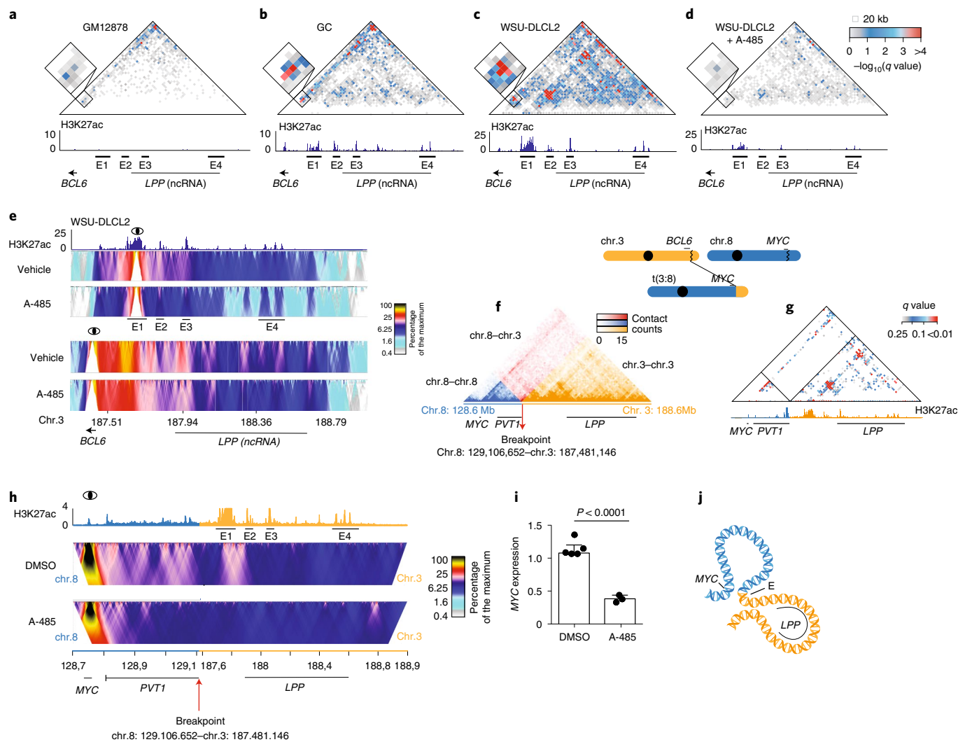
Fig. 5 | Enhancer region on chr.3 regulates the expression of BCL6 and MYC . a–d , Representation of 20-kb interacting regions between the indicated genomic coordinates with a zoom-in in the region between BCL6 and E1 enhancer regions (top) and corresponding ChIP-seq track of H3K27ac in GM12878 (n.r.p.m.; a ), GC (n.r.p.m.; b ) and WSU-DLCL2 cells untreated (r.r.p.m.; c ) or treated with A-485 inhibitor (r.r.p.m.; d ). The 20-kb regions in the interacting maps are color coded based on their q value. The enhancer regions detected in lymphoma cells have been labeled with progressive numbers (E1, E2, E3, E4). e , The UMI-4C domainogram using two different bait primers and the corresponding H3K27ac ChIP-seq track (r.r.p.m.) in WSU-DLCL2 cells treated with A-485 (0.5 \mu M for 48 h) or vehicle (DMSO) as a control. The eye represents the position of the primer used as bait. f , Graphic representation of the chromosomal translocation t(3;8) between the indicated regions on chr.3 and chr.8, and reconstruction of Hi-C contact maps of the derivative chromosome t(3;8) in the region spanning the breakpoint after chromosomal translocation in WSU-DLCL2. The chr.3 intrachromosomal contacts are in yellow, chr.8 intrachromosomal contacts are in blue and the interchromosomal interactions between chr.3 and chr.8 are in red. g , Representation of 20-kb regions significantly interacting color coded based on their q values in the derivative chromosome t(3;8) (top) and reconstruction of the H3K27ac ChIP-seq tracks (n.r.p.m.) in WSU-DLCL2 cells (bottom). h , UMI-4C domainogram representing the mean number of contacts (percentage of the maximum) spanning the breakpoint after chromosomal translocation between chr.8 and chr.3 in WSU-DLCL2 cells treated with A-485 (0.5 \mu M for 48 h) or DMSO as control and the corresponding H3K27ac ChIP-seq track in untreated cells. The eye represents the position of the primer used as bait. i , Quantification of MYC expression changes on treatment with A-485 0.5 \mu M for 48 h in WSU-DLCL2 ( n=3 ) compared with the same cells treated with DMSO (vehicle n=5 ). Data are presented as mean \pm s.d. The P value was calculated using an unpaired, two-tailed Student's t -test. j , Graphic representation of chromatin conformation on translocation between chr.8 in blue and chr.3 in yellow.
