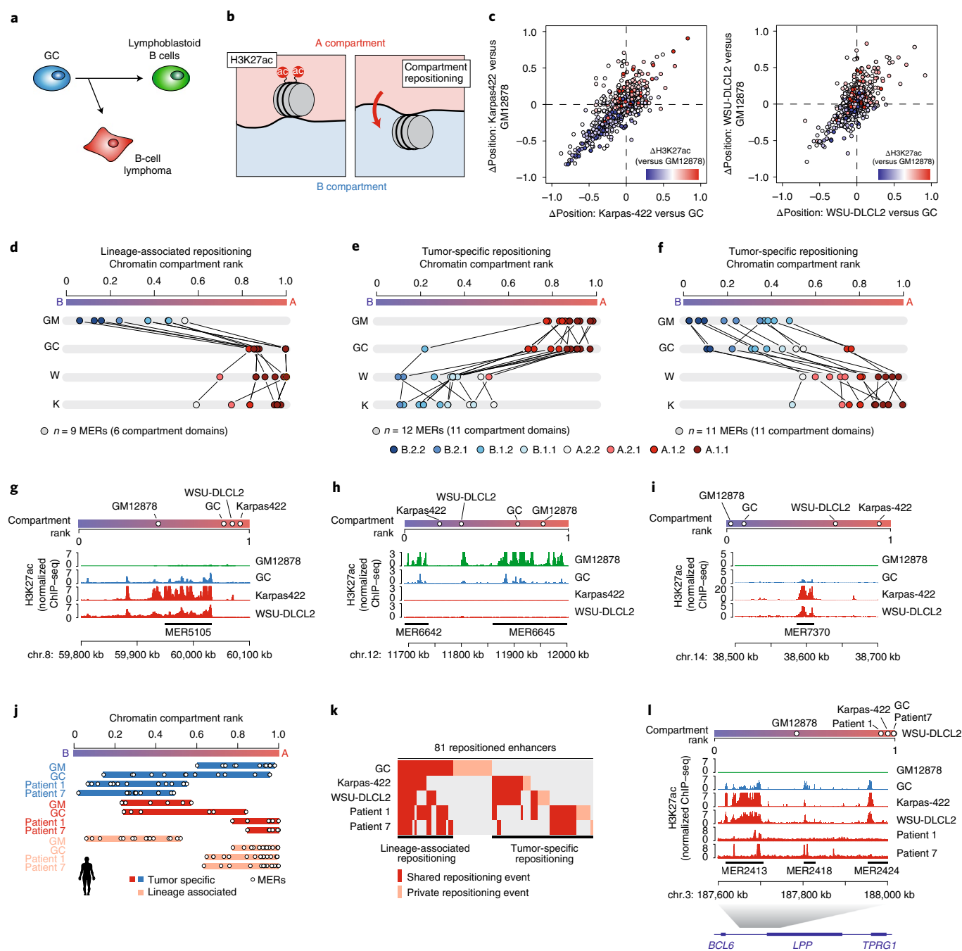
Fig. 1 | Repositioning of enhancer regions in chromatin subcompartment domains. a , Graphic representation of the models used in the present study. Arrows indicate differentiation and tumor development trajectories. b , Graphic representation of repositioning of enhancer regions between A and B compartments that accompany changes in H3K27ac. c , Comparison of compartment domain rank differences computed with Calder between (left) Karpas-422 and GC cells (x axis) and Karpas-422 and GM12878 (y axis) and between (right) WSU-DLCL2 and GC cells (x axis) and WSU-DLCL2 and GM12878 (y axis). Each dot is an MER color coded by the difference in H3K27ac between Karpas-422 (left) or WSU-DLCL2 (right) and GM12878 (red: higher H3K27ac in lymphoma cell lines than in GM12878; blue: lower H3K27ac in lymphoma cell lines than in GM12878). d-f , Compartment domain rank (x axis) of enhancer regions in cancer cell lines (WSU-DLCL2 (W) and Karpas-422 (K)) and normal B cells (GC and GM12878 (GM)). From left to right: enhancer regions exhibiting lineage-specific repositioning ( d ), and enhancer regions exhibiting tumor-specific repositioning toward inactive ( e ) or active ( f ) subcompartments. Each dot is an enhancer region and color coded by subcompartment assignment. g-i , Representative examples of H3K27ac ChIP-seq tracks of enhancer regions and their position in the compartment rank in the indicated samples (top bar) indicating lineage associated repositioning on chr.8 ( g ), and tumor specific repositioning chr.12 ( h ) and chr.14 ( i ). j , Compartment domain rank (x axis) of enhancer regions in lymphoma primary patient samples (patients 1 and 7) and normal B cells (GC and GM12878). k , Occurrence of repositioned enhancer regions in the indicated samples compared with GM12878. Shared repositioning events are observed in at least two samples. Private repositioning events are observed in only one sample. l , H3K27ac ChIP-seq tracks of the indicated region on chr.3 and its position in the compartment rank in the indicated samples. The ChIP-seq scale is reported as normalized reads per million (n.r.p.m.) for cell lines and reference-adjusted reads per million (r.r.p.m.) \times 10^{-2} for patient samples. The position of this region in the larger genomic locus, comprising the BCL6 , LPP and TPRG1 genes, is shown at the bottom.
