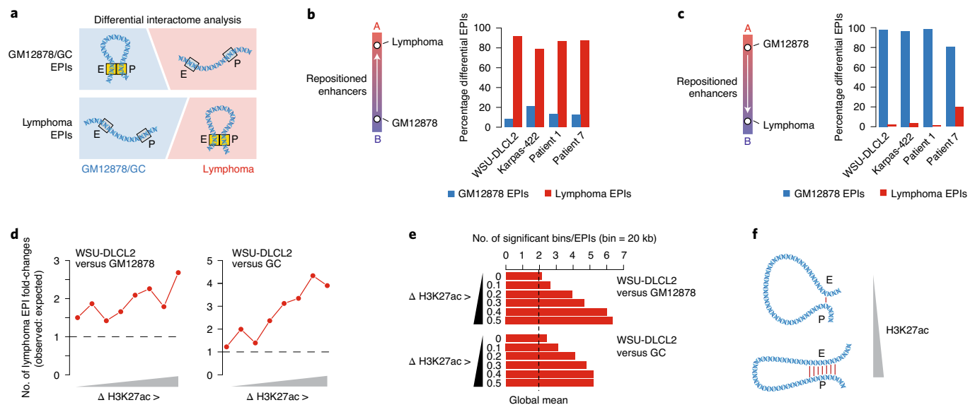
Fig. 2 | Changes in H3K27ac modulate the frequency and size of EPIs. a , Graphic representation of the differential interactome analysis. The presence (DNA loop with yellow boxes) and absence (DNA string with gray boxes) of EPIs is compared between normal B cells (GM12878 and GC in blue) and lymphoma cells (red), including both cell lines and primary samples. E, enhancer; P, promoter. b,c , Percentage of significantly different EPIs (y axis), which are more frequent either in GM12878 than in the indicated lymphoma samples (blue bars) or in lymphoma samples than in GM12878 (red bars). Results are shown for enhancer regions that were repositioned from inactive to active compartment ( b ) or from active to inactive compartment ( c ) in lymphoma samples with respect to GM12878. d , Fold-change between the observed and expected number of significantly more frequent EPIs (y axis) in WSU-DLCL2 than GM12878 (left) and GC (right), with respect to the difference in H3K27ac in these regions. e , Number of significant interactions per EPI (that is, number of bins of the Hi-C map with significantly frequent interactions between the enhancer and promoter regions; x axis), with respect to the difference in H3K27ac in these regions. Results are shown for EPIs that were more frequent in WSU-DLCL2 than in GM12878 (top) or in GC (bottom). f , Graphic representation of the changes in EPI conformation as a consequence of increased H3K27ac considering the number of bins and frequency (represented as red lines) of interactions.
