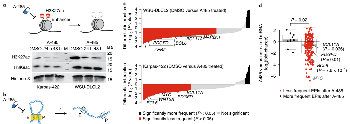
Fig. 3 | Reduction of H3K27ac modulates the frequency and the size of EPIs. a , Graphic representation of experimental design on treatment with A-485 inhibitor (top) and a representative western blot image ( n = 2 independent experiments) detecting the indicated histone post-translational modifications and histone H3 in Karpas-422 and WSU-DLCL2 treated with dimethylsulfoxide (DMSO; vehicle) or A-485 (0.5 \mu M) for 24 h and 48 h (bottom). b , Graphic representation of EPI comparison before and after A-485 treatment. A-485 treatment is hypothesized to induce loss of EPIs. E, enhancer; P, promoter. c , Differential interactome significance (y axis) of EPIs before and after A-485 treatment: EPIs were either significantly (DiffInt P < 0.05 ) more frequent (black) or less frequent (red) on treatment with A-485 or similarly frequent (not significant—gray) in WSU-DLCL2 (top) and Karpas-422 (bottom). d , The mRNA expression fold-changes between A-485-treated and untreated lymphoma cells of genes in which EPIs are less frequent (red) or more frequent (black) on treatment. Fold-changes are computed for both lymphoma cell lines (Karpas-422 and WSU-DLCL2), each analyzed in triplicate. The thick central line in the box plot represents the median value, the bounding box corresponds to the 25th–75th percentiles and the whiskers extend up to 1.5× the interquartile range. Representative genes are labeled. The P value was computed using two-tailed Wilcoxon's test.
