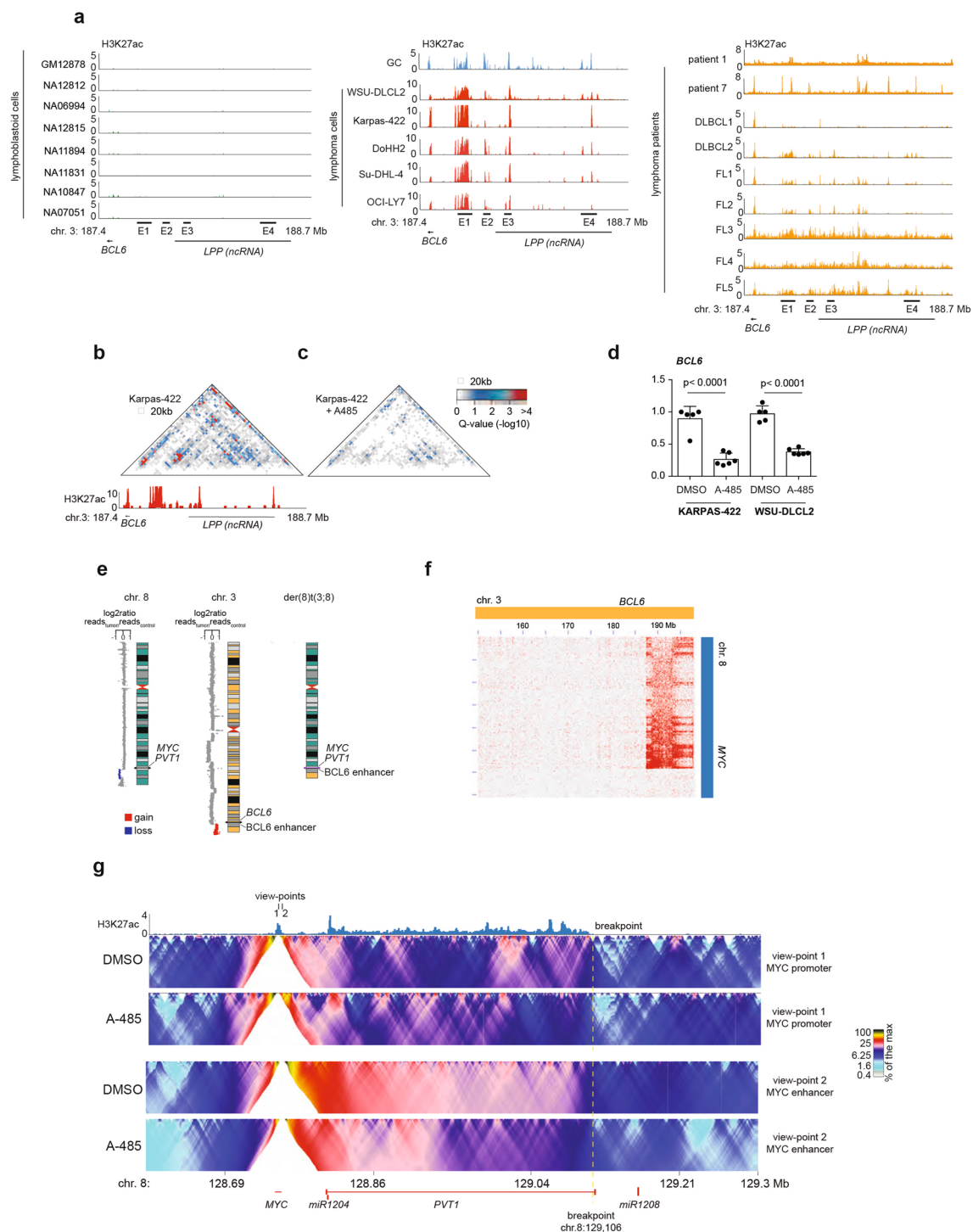
Extended Data Fig. 5 | Analyses of the chromatin structure in BCL6 and MYC loci. a , Representative ChIP sequencing tracks of H3K27ac in lymphoblastoid cells, GC, DLBCL tumor cells, and in primary lymphoma samples (NRPM), Patient 1 and Patient 7 are reported as RRPm \times 10^{-2} . b-c , Representation of 20kb interacting regions in chr.3 187.4–188.7 Mb color coded based on their q value (top) in Karpas-422 untreated ( b ) or treated with A-485 inhibitor ( c ) and corresponding H3K27ac ChIP-sequencing (NRPM). d , Quantification of expression changes of BCL6 upon treatment with A-485 0.5 \mu M for 48h in Karpas-422 (n=6) and WSU-DLCL2 (n=6) compared to the same cells treated with DMSO (vehicle, n=5). The black dots represent the number of independent experiments. Data are presented as mean value + SD. p-value were calculated using unpaired two-tailed t-test. e , Representation of copy number changes detected on chr. 8 and chr. 3 and graphical representation of the derivative chromosome t(3;8). f , Hi-C inter-chromosomal contact maps of chr.8 and chr.3 in the region spanning the breakpoint in WSU-DLCL2 cells. g , ChIP-sequencing track of H3K27ac (blue, NRPM) and UMI-4C domainogram with two different bait-primers representing the mean number of contacts (% of the maximum) on chr.8 spanning the breakpoint in WSU-DLCL2 cells treated with A-485 (0.5 \mu M for 48h) or DMSO as control.
