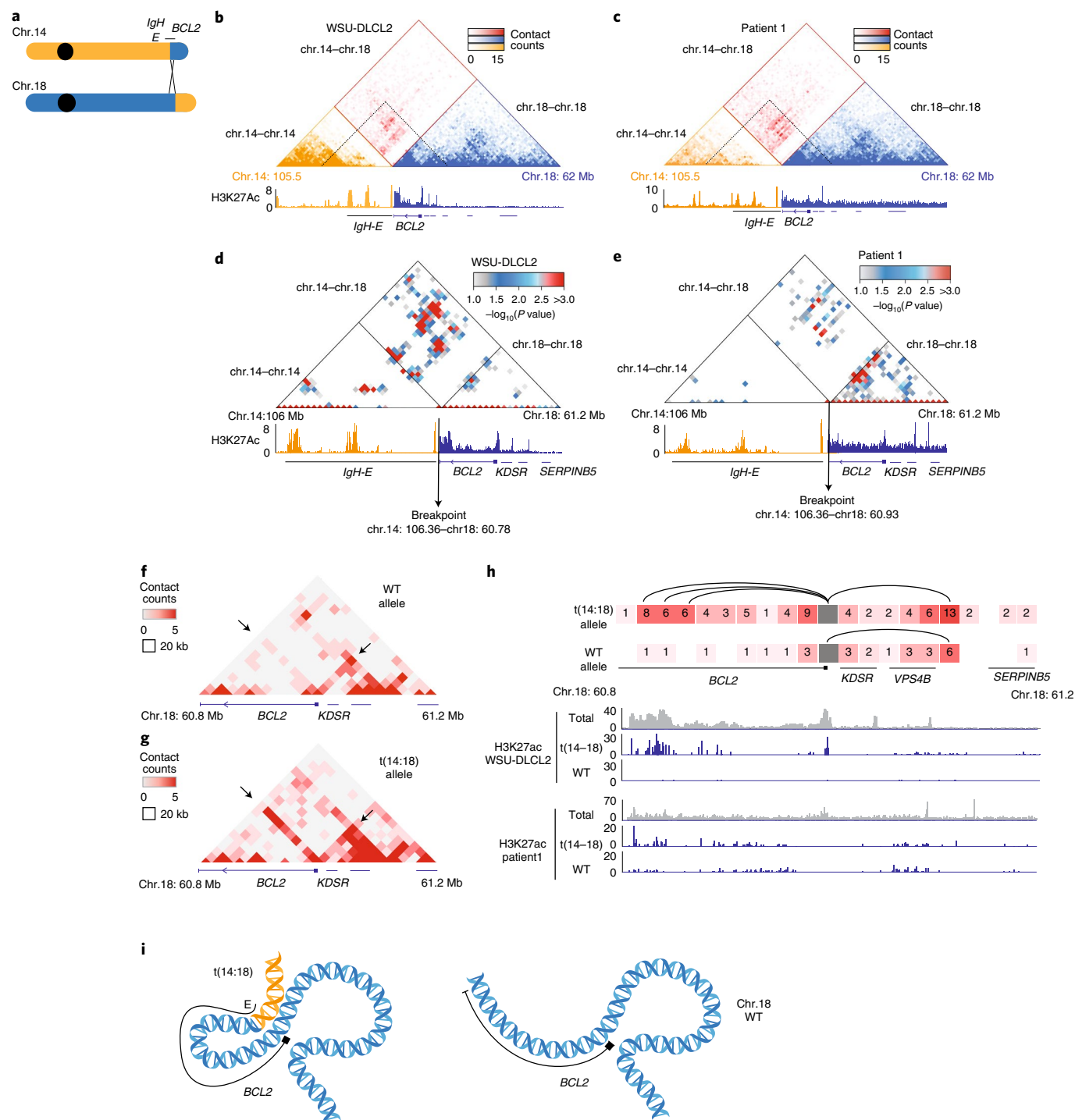
Fig. 7 | Allele-specific epigenetic marks and chromatin interactions at the BCL2 locus. a , Graphic representation of the chromosomal translocation t(14;18). b, c , Reconstruction of Hi-C contact maps of the derivative chromosome t(14;18) in the region spanning the breakpoint after chromosomal translocation in WSU-DLCL2 ( b ) and patient 1 ( c ). The chr.14 intrachromosomal contacts are in yellow, chr.18 intrachromosomal contacts in blue and interchromosomal interactions between chr.14 and chr.18 in red. The dotted lines indicate the region represented in d and e . d, e , Representation of 20-kb regions significantly interacting are color coded based on their P values in the derivative chromosome t(14;18) and reconstruction of the corresponding H3K27ac ChIP-seq tracks in WSU-DLCL2 cells (n.r.p.m.; d ) and patient 1 (r.r.p.m. \times 10^{-2} ; e ). P values obtained with the HiC-DC method are represented. f, g , Representation of allele-specific Hi-C interactions in the region containing the BCL2 WT allele and BCL2 -translocated t(14;18) allele. h , Quantification of the Hi-C reads starting from the 20-kb bins containing the BCL2 promoter in the WT and translocated t(14;18) allele (top) and distribution of H3K27ac ChIP-seq tracks in the corresponding WT and translocated t(14;18) chromosome in WSU-DLCL2 cells and patient 1 (bottom). The H3K27ac distribution of the total signal is in gray. The number of reads in each 20-kb bin is indicated. i , Graphic representation of chromatin conformation of BCL2 WT and translocated alleles on the two copies of chr.18.
