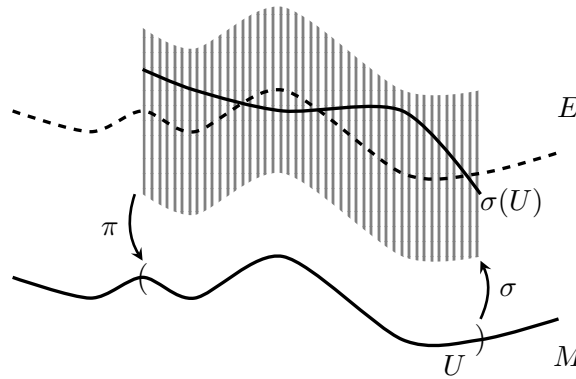
Figure 6.2: A local section of a vector bundle
